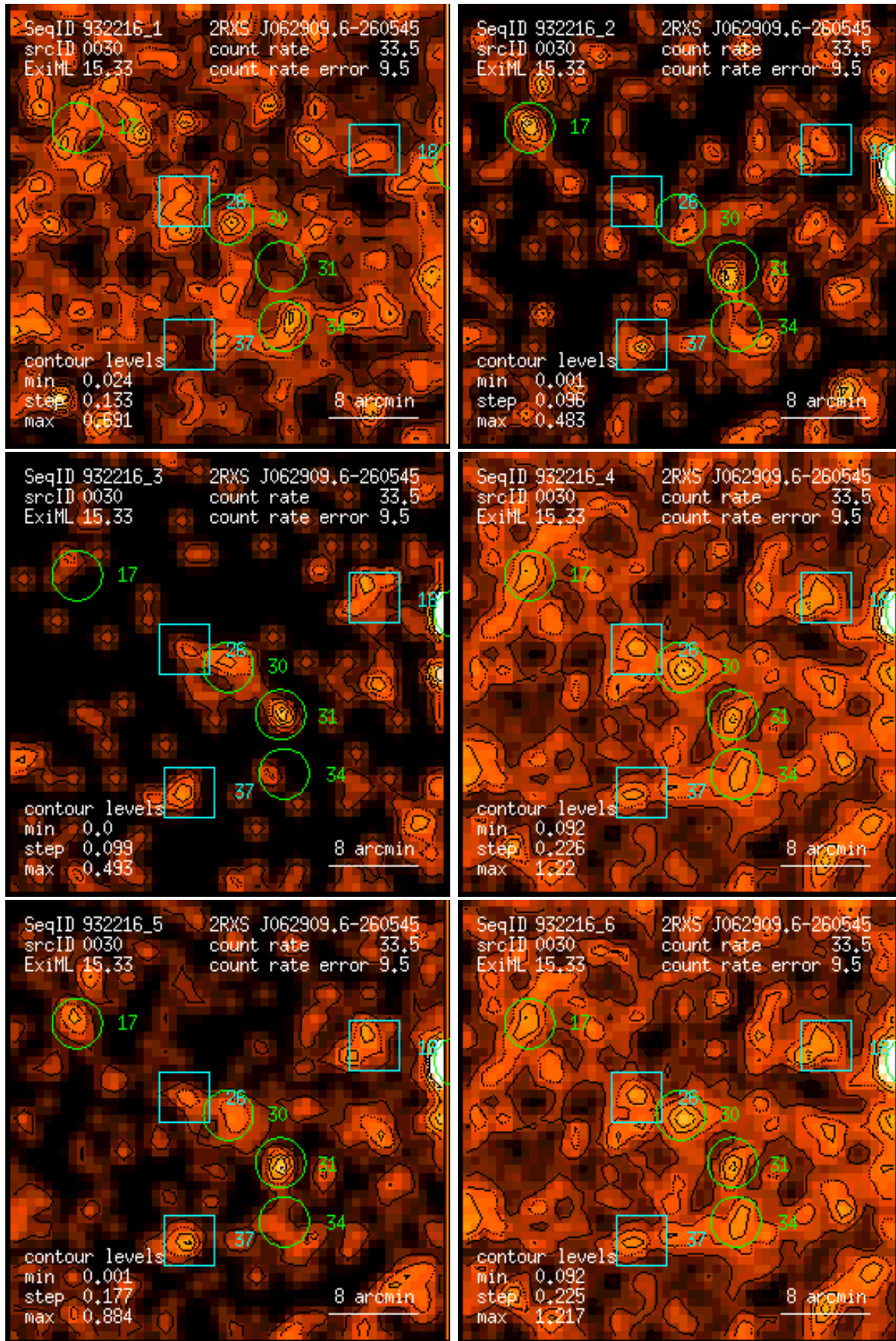
Figure 30: RASS 932216: detection 0030: band rate images, Gaussian filter: (1) PSPC channels 11 – 41, (2) 52 – 90, (3) 91 – 201, (4) 11 – 235, (5) 52 – 201, (6) 11 – 201. Broad band rates in counts/ks. Band rate contour levels in counts/ks/arcmin 2 .
