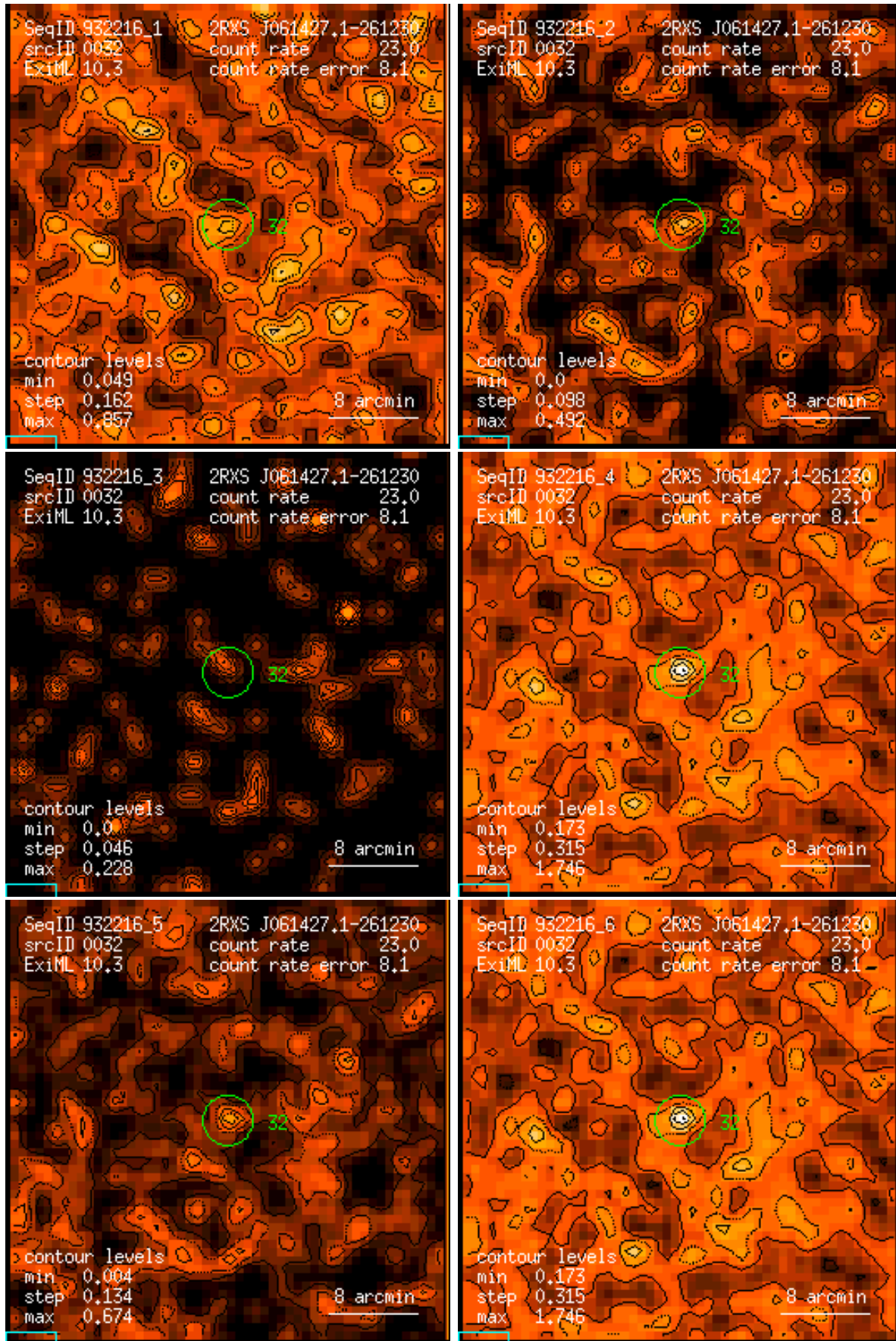
Figure 32: RASS 932216: detection 0032: band rate images, Gaussian filter: (1) PSPC channels 11 – 41, (2) 52 – 90, (3) 91 – 201, (4) 11 – 235, (5) 52 – 201, (6) 11 – 201. Broad band rates in counts/ks. Band rate contour levels in counts/ks/arcmin 2 .
