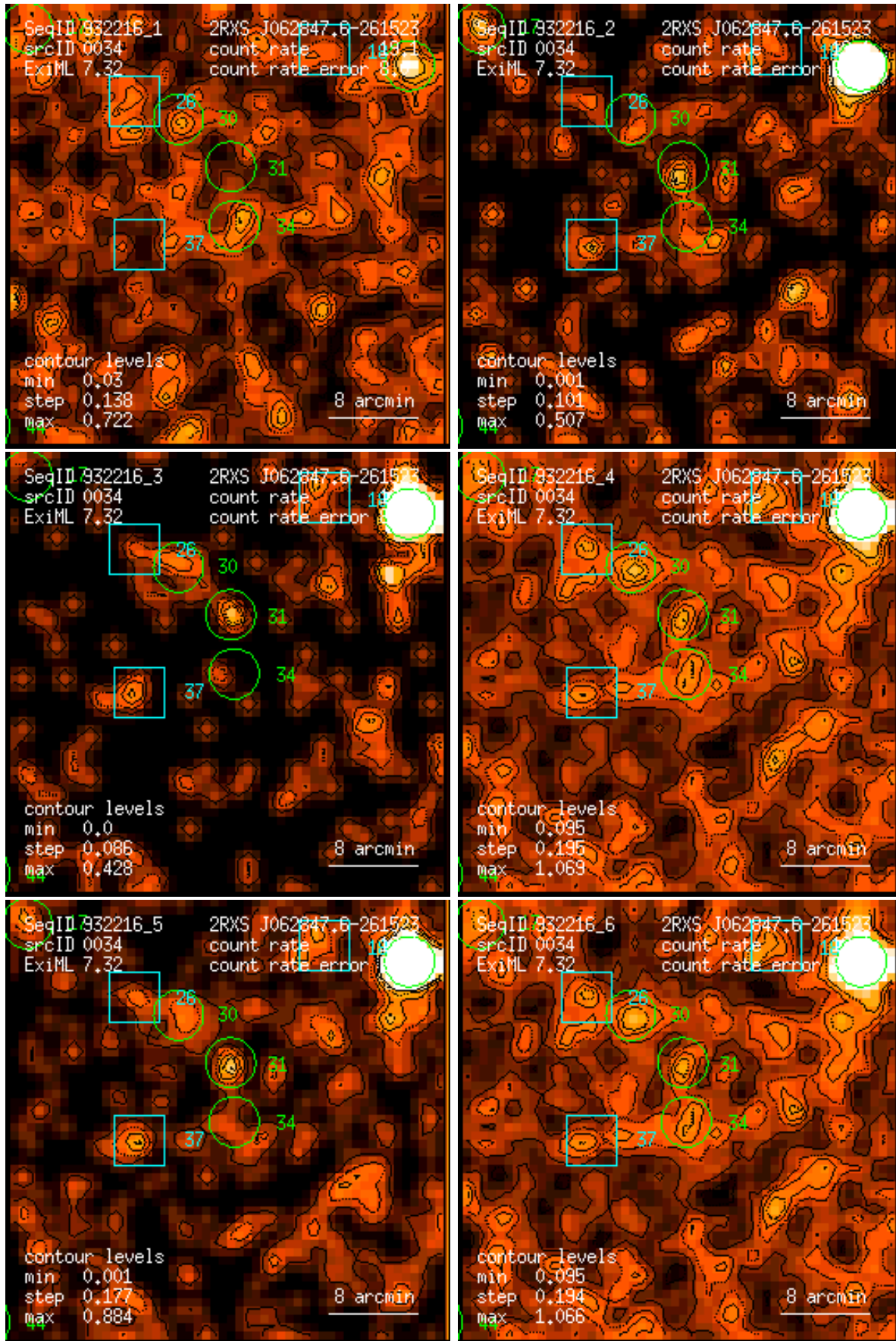
Figure 34: RASS 932216: detection 0034: band rate images, Gaussian filter: (1) PSPC channels 11 – 41, (2) 52 – 90, (3) 91 – 201, (4) 11 – 235, (5) 52 – 201, (6) 11 – 201. Broad band rates in counts/ks. Band rate contour levels in counts/ks/arcmin 2 .
