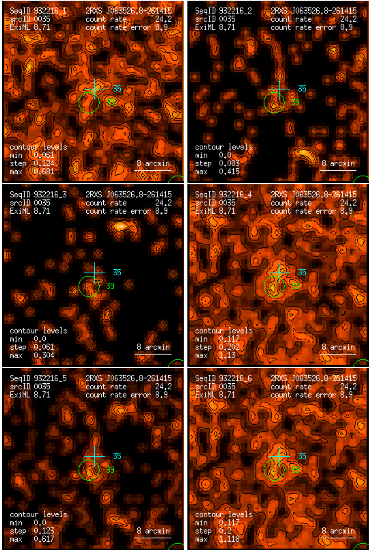
Figure 35: RASS 932216: detection 0035: band rate images, Gaussian filter: (1) PSPC channels 11 – 41, (2) 52 – 90, (3) 91 – 201, (4) 11 – 235, (5) 52 – 201, (6) 11 – 201. Broad band rates in counts/ks. Band rate contour levels in counts/ks/arcmin 2 .
