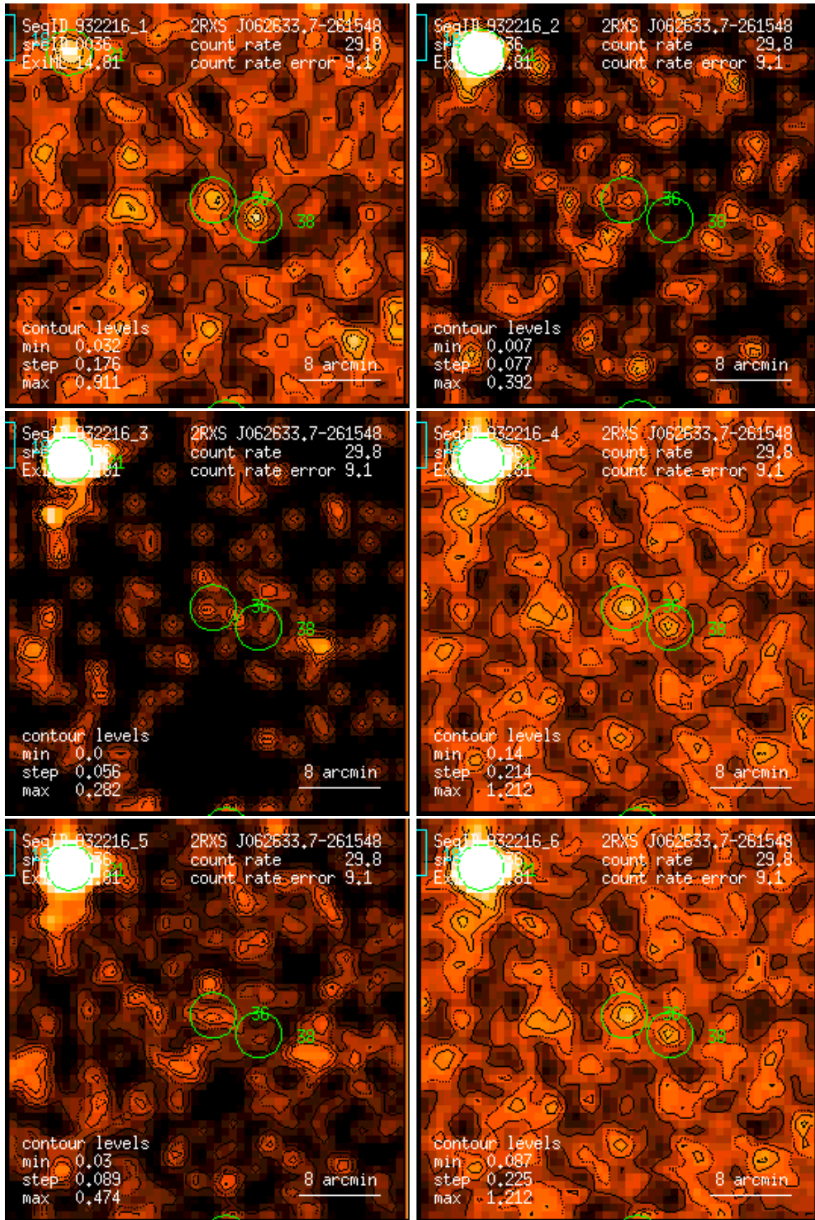
Figure 36: RASS 932216: detection 0036: band rate images, Gaussian filter: (1) PSPC channels 11 – 41, (2) 52 – 90, (3) 91 – 201, (4) 11 – 235, (5) 52 – 201, (6) 11 – 201. Broad band rates in counts/ks. Band rate contour levels in counts/ks/arcmin 2 .
