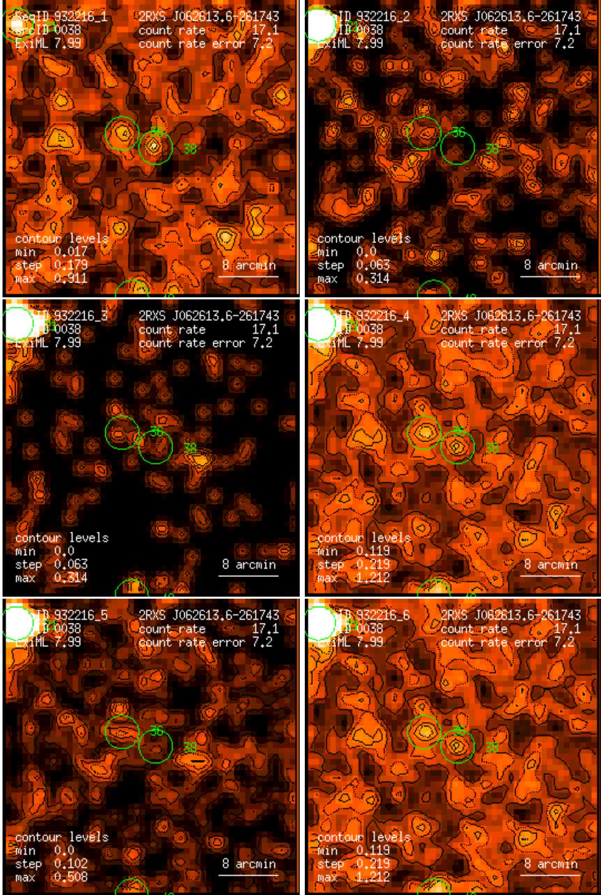
Figure 38: RASS 932216: detection 0038: band rate images, Gaussian filter: (1) PSPC channels 11 – 41, (2) 52 – 90, (3) 91 – 201, (4) 11 – 235, (5) 52 – 201, (6) 11 – 201. Broad band rates in counts/ks. Band rate contour levels in counts/ks/arcmin 2 .
