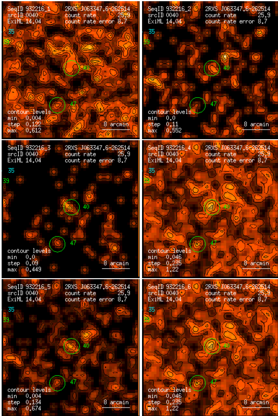
Figure 40: RASS 932216: detection 0040: band rate images, Gaussian filter: (1) PSPC channels 11 – 41, (2) 52 – 90, (3) 91 – 201, (4) 11 – 235, (5) 52 – 201, (6) 11 – 201. Broad band rates in counts/ks. Band rate contour levels in counts/ks/arcmin 2 .
