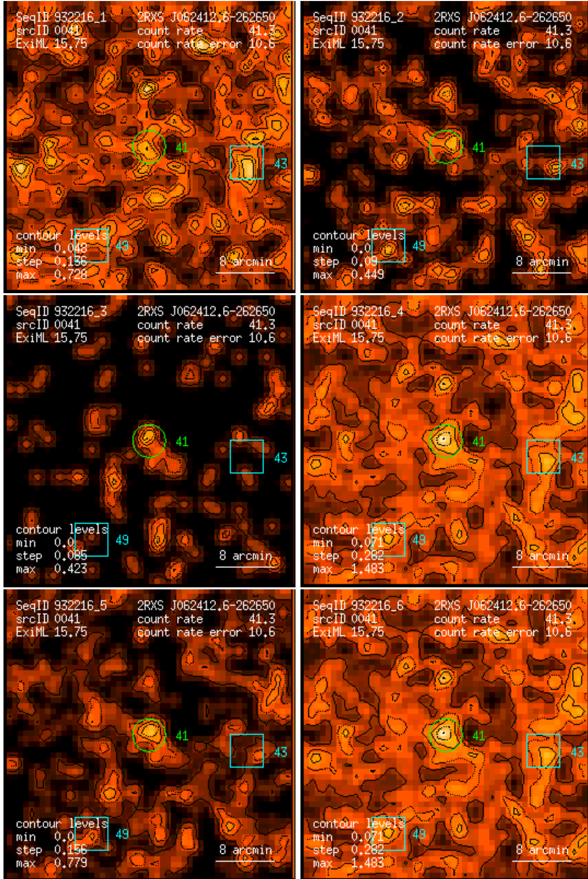
Figure 41: RASS 932216: detection 0041: band rate images, Gaussian filter: (1) PSPC channels 11 – 41, (2) 52 – 90, (3) 91 – 201, (4) 11 – 235, (5) 52 – 201, (6) 11 – 201. Broad band rates in counts/ks. Band rate contour levels in counts/ks/arcmin 2 .
