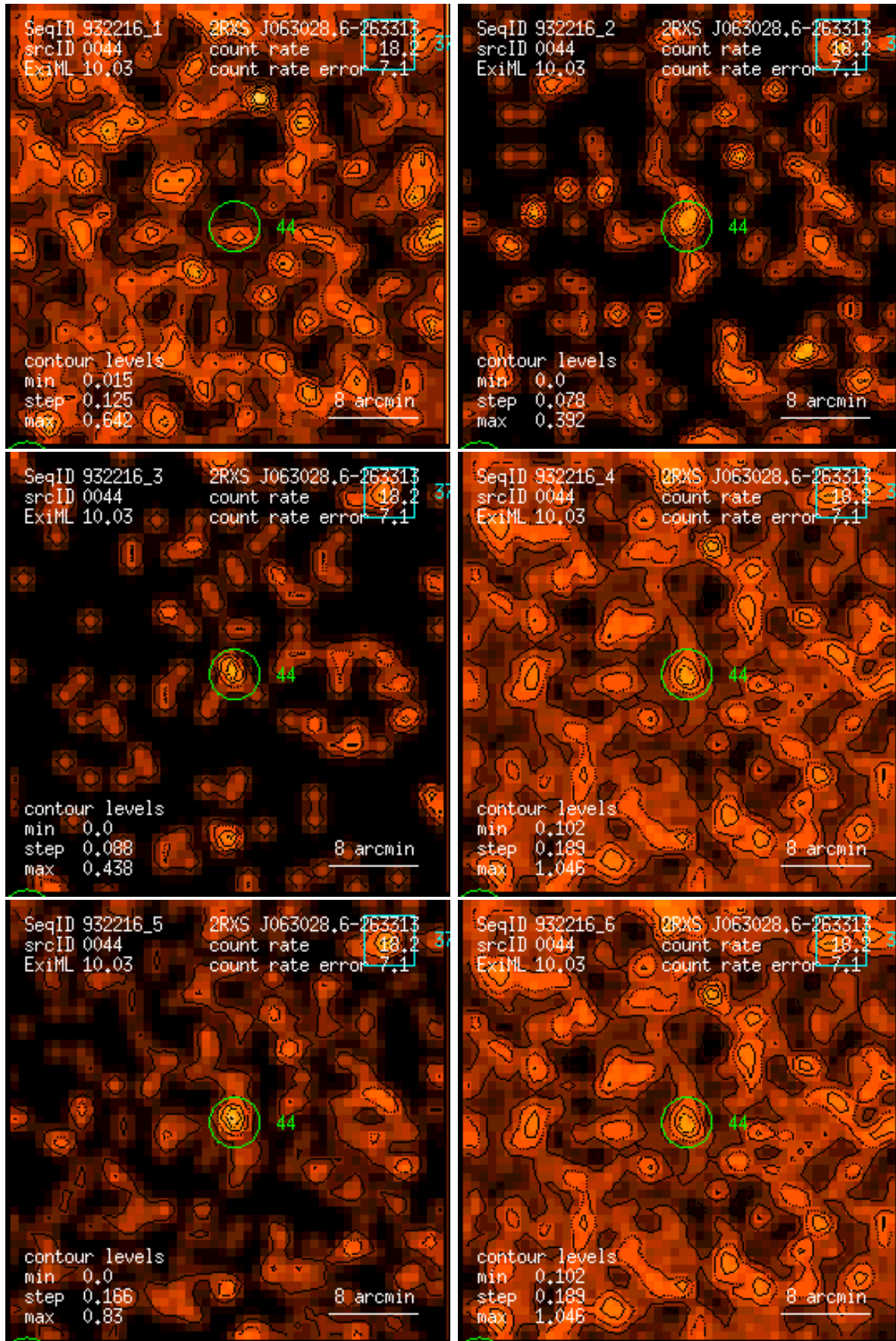
Figure 44: RASS 932216: detection 0044: band rate images, Gaussian filter: (1) PSPC channels 11 – 41, (2) 52 – 90, (3) 91 – 201, (4) 11 – 235, (5) 52 – 201, (6) 11 – 201. Broad band rates in counts/ks. Band rate contour levels in counts/ks/arcmin 2 .
