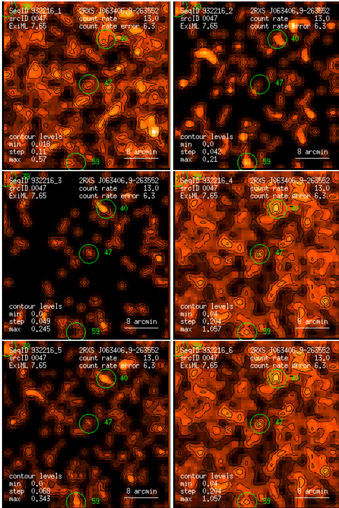
Figure 47: RASS 932216: detection 0047: band rate images, Gaussian filter: (1) PSPC channels 11 – 41, (2) 52 – 90, (3) 91 – 201, (4) 11 – 235, (5) 52 – 201, (6) 11 – 201. Broad band rates in counts/ks. Band rate contour levels in counts/ks/arcmin 2 .
