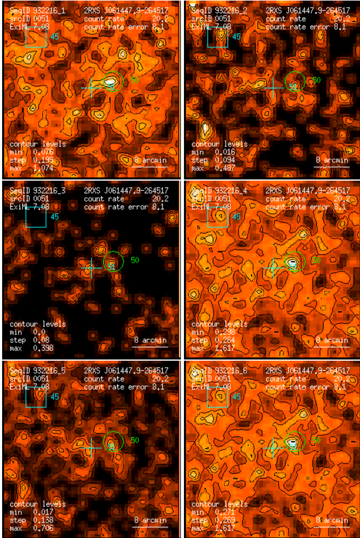
Figure 51: RASS 932216: detection 0051: band rate images, Gaussian filter: (1) PSPC channels 11 – 41, (2) 52 – 90, (3) 91 – 201, (4) 11 – 235, (5) 52 – 201, (6) 11 – 201. Broad band rates in counts/ks. Band rate contour levels in counts/ks/arcmin 2 .
