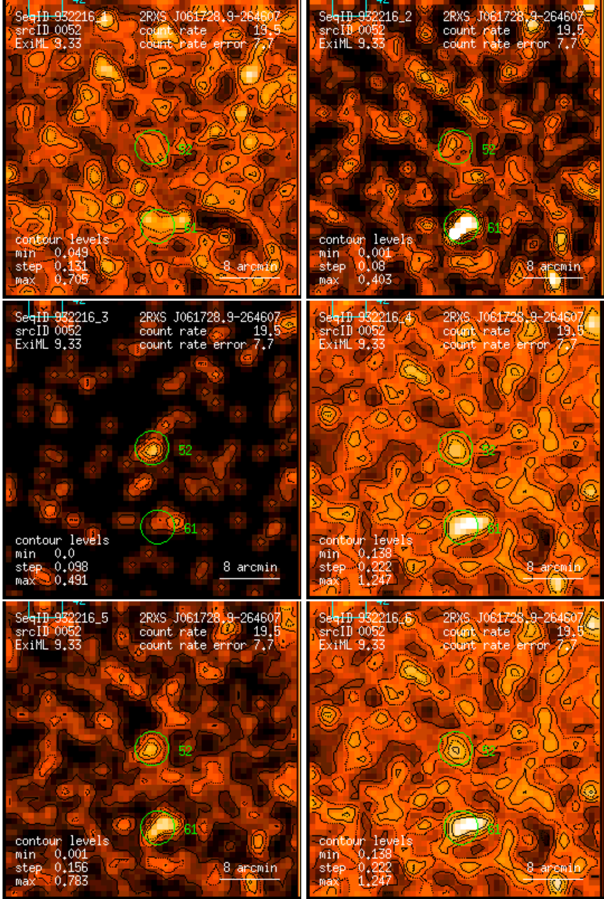
Figure 52: RASS 932216: detection 0052: band rate images, Gaussian filter: (1) PSPC channels 11 – 41, (2) 52 – 90, (3) 91 – 201, (4) 11 – 235, (5) 52 – 201, (6) 11 – 201. Broad band rates in counts/ks. Band rate contour levels in counts/ks/arcmin 2 .
