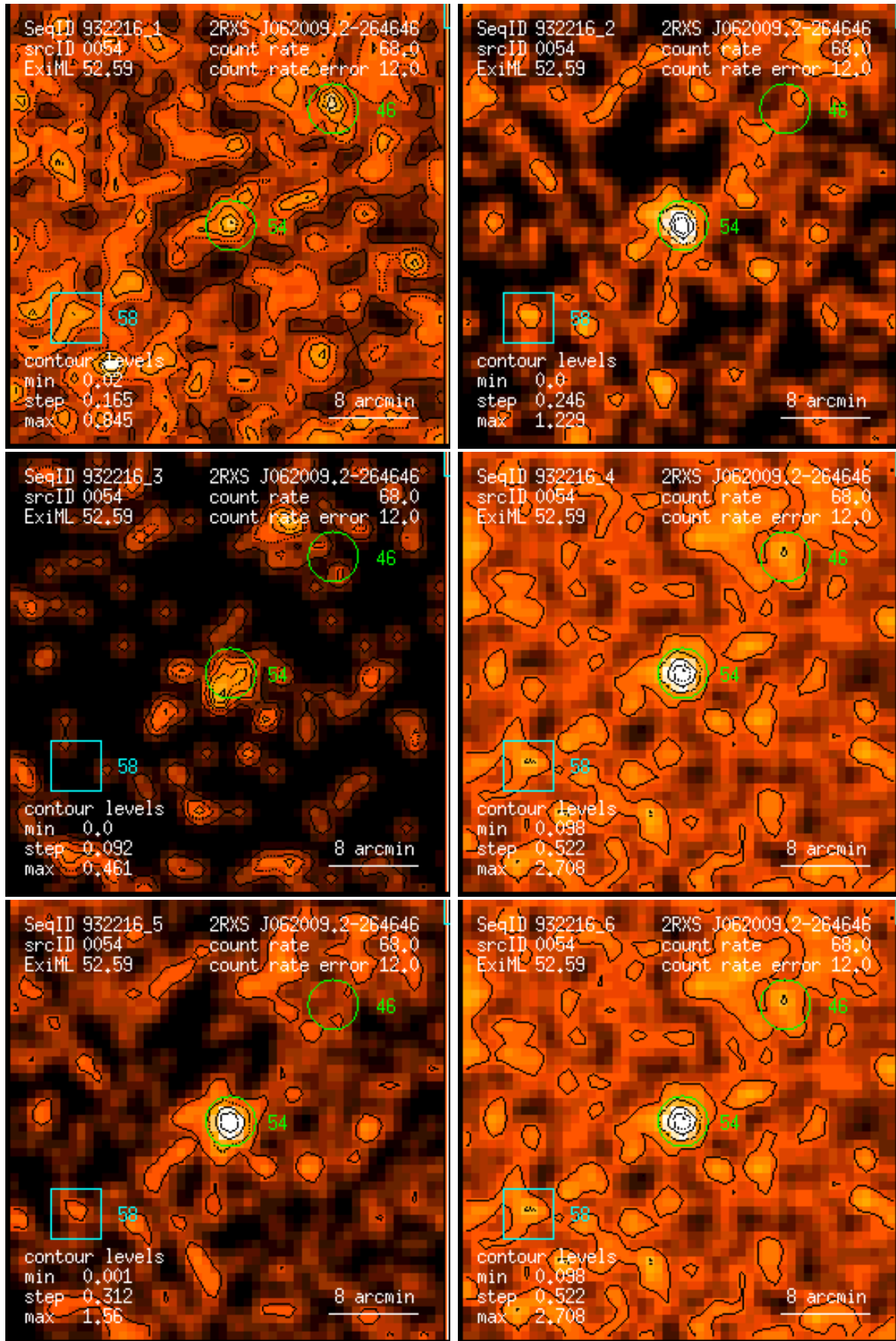
Figure 54: RASS 932216: detection 0054: band rate images, Gaussian filter: (1) PSPC channels 11 – 41, (2) 52 – 90, (3) 91 – 201, (4) 11 – 235, (5) 52 – 201, (6) 11 – 201. Broad band rates in counts/ks. Band rate contour levels in counts/ks/arcmin 2 .
