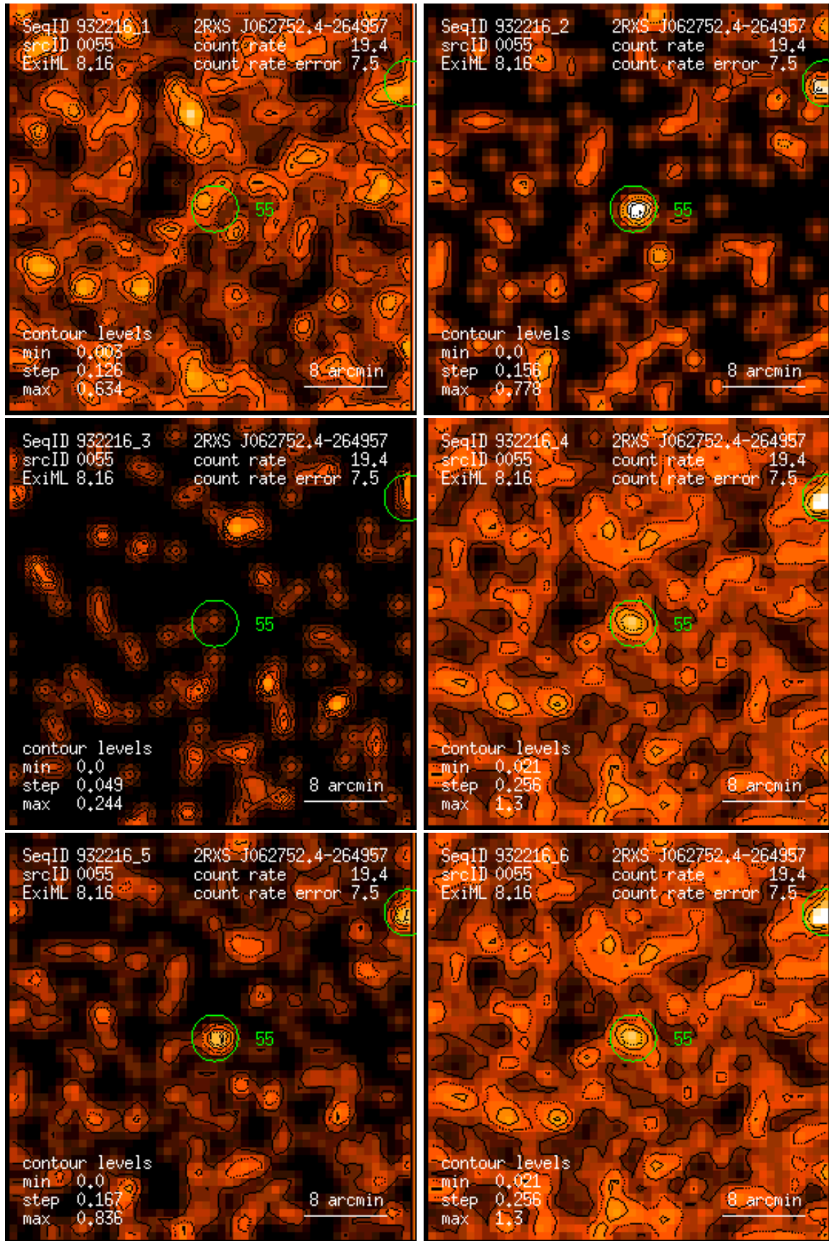
Figure 55: RASS 932216: detection 0055: band rate images, Gaussian filter: (1) PSPC channels 11 – 41, (2) 52 – 90, (3) 91 – 201, (4) 11 – 235, (5) 52 – 201, (6) 11 – 201. Broad band rates in counts/ks. Band rate contour levels in counts/ks/arcmin 2 .
