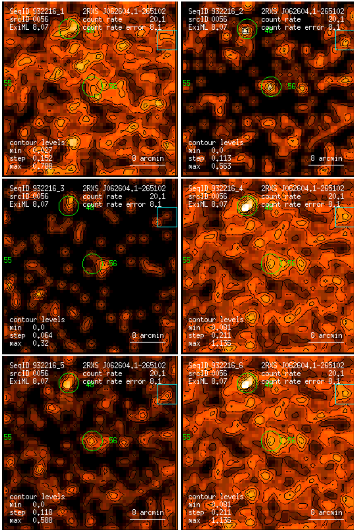
Figure 56: RASS 932216: detection 0056: band rate images, Gaussian filter: (1) PSPC channels 11 – 41, (2) 52 – 90, (3) 91 – 201, (4) 11 – 235, (5) 52 – 201, (6) 11 – 201. Broad band rates in counts/ks. Band rate contour levels in counts/ks/arcmin 2 .
