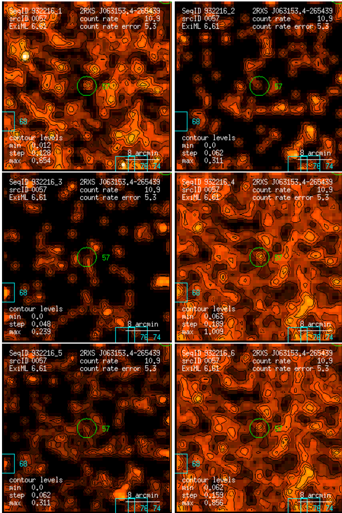
Figure 57: RASS 932216: detection 0057: band rate images, Gaussian filter: (1) PSPC channels 11 – 41, (2) 52 – 90, (3) 91 – 201, (4) 11 – 235, (5) 52 – 201, (6) 11 – 201. Broad band rates in counts/ks. Band rate contour levels in counts/ks/arcmin 2 .
