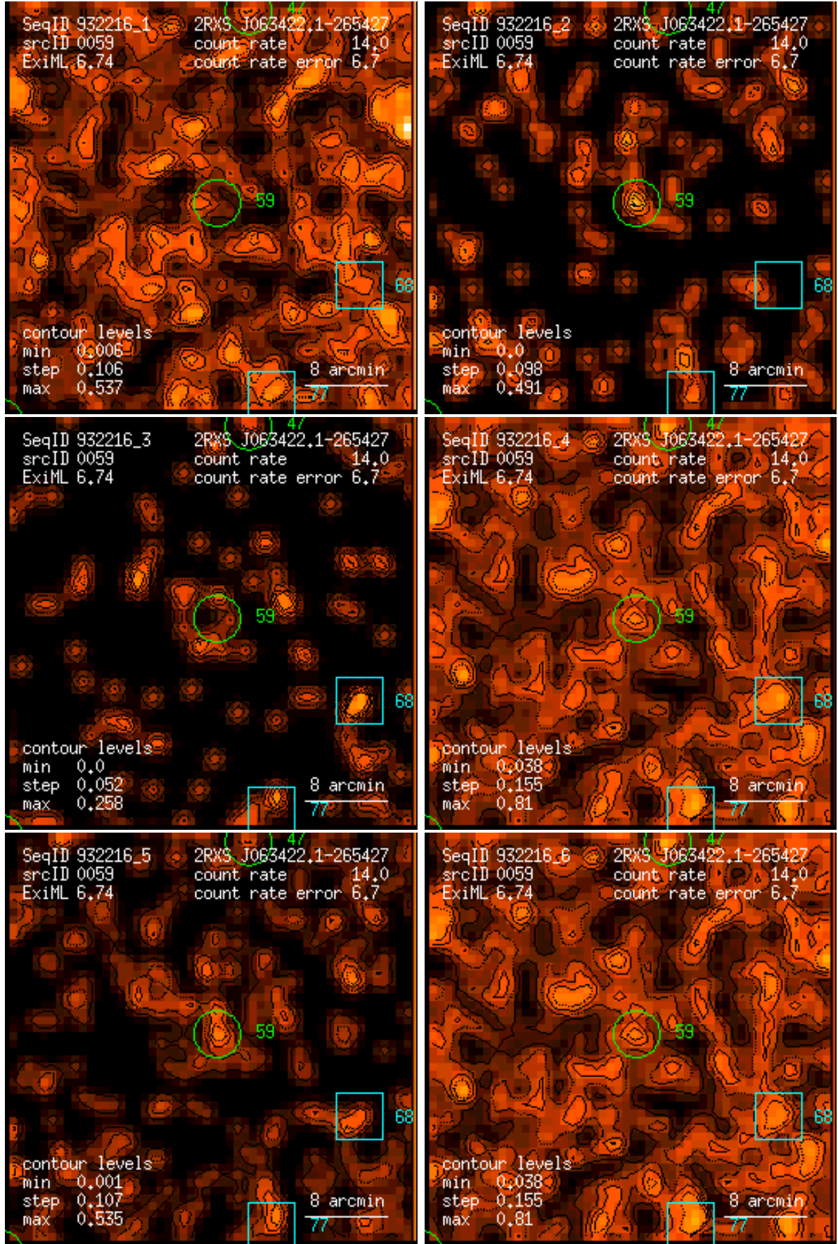
Figure 59: RASS 932216: detection 0059: band rate images, Gaussian filter: (1) PSPC channels 11 – 41, (2) 52 – 90, (3) 91 – 201, (4) 11 – 235, (5) 52 – 201, (6) 11 – 201. Broad band rates in counts/ks. Band rate contour levels in counts/ks/arcmin 2 .
