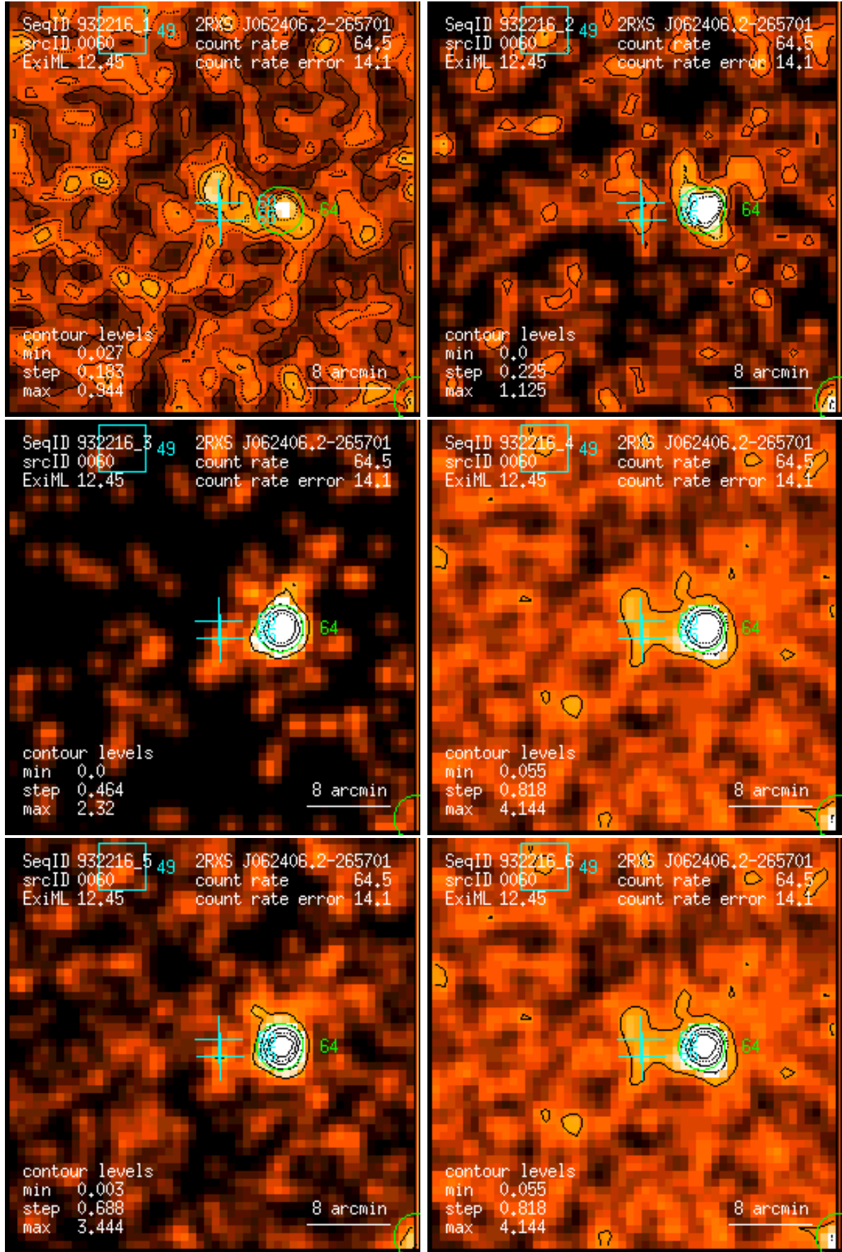
Figure 60: RASS 932216: detection 0060: band rate images, Gaussian filter: (1) PSPC channels 11 – 41, (2) 52 – 90, (3) 91 – 201, (4) 11 – 235, (5) 52 – 201, (6) 11 – 201. Broad band rates in counts/ks. Band rate contour levels in counts/ks/arcmin 2 .
