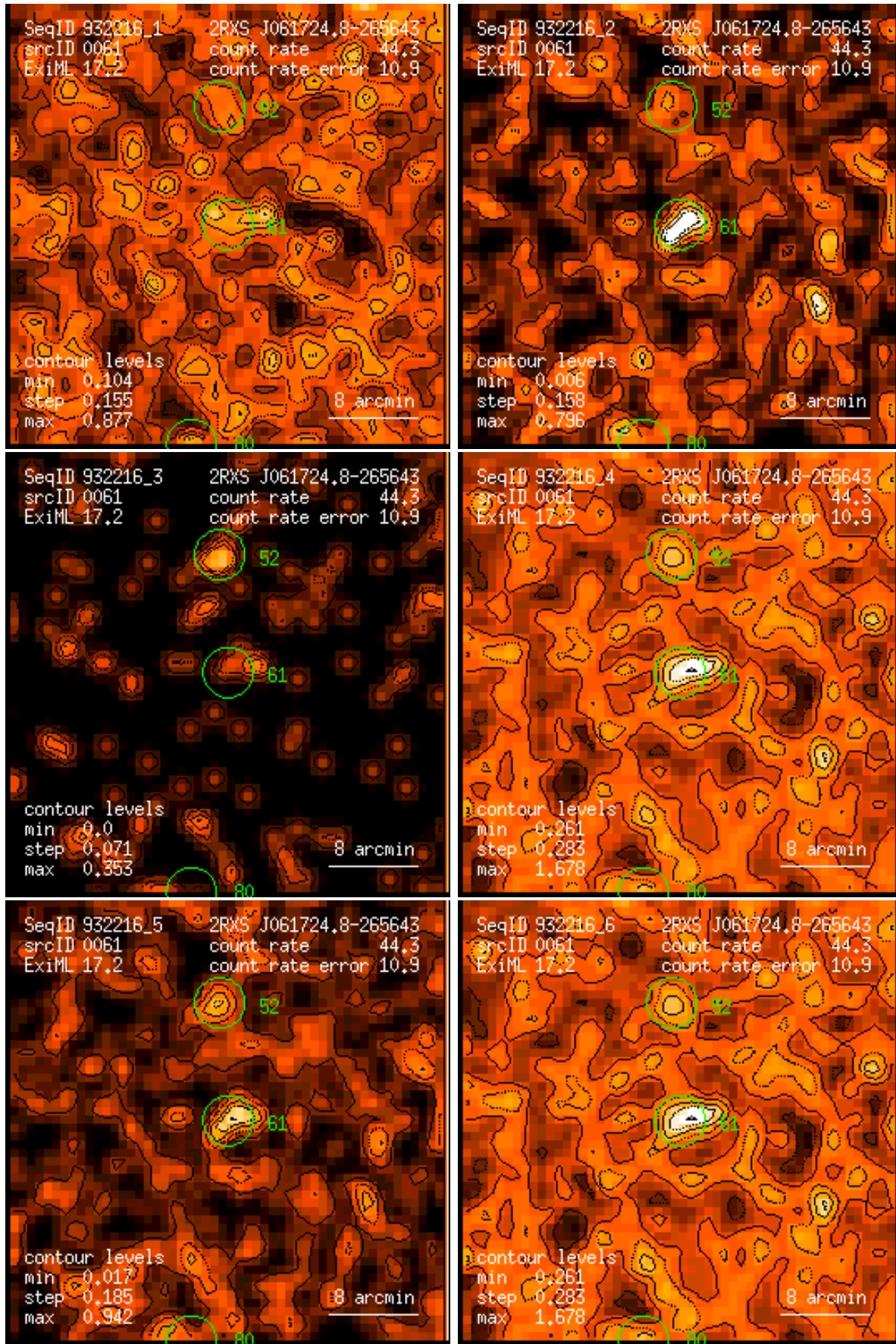
Figure 61: RASS 932216: detection 0061: band rate images, Gaussian filter: (1) PSPC channels 11 – 41, (2) 52 – 90, (3) 91 – 201, (4) 11 – 235, (5) 52 – 201, (6) 11 – 201. Broad band rates in counts/ks. Band rate contour levels in counts/ks/arcmin 2 .
