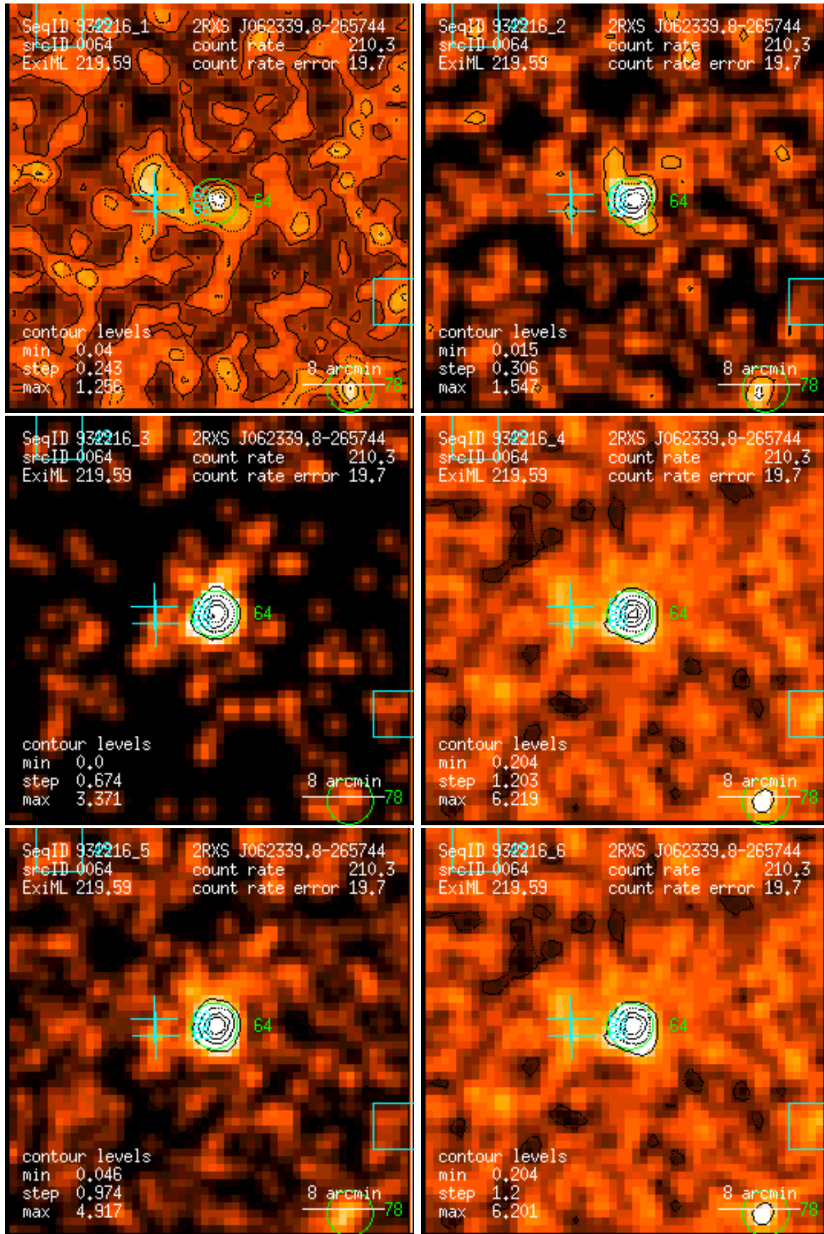
Figure 64: RASS 932216: detection 0064: band rate images, Gaussian filter: (1) PSPC channels 11 – 41, (2) 52 – 90, (3) 91 – 201, (4) 11 – 235, (5) 52 – 201, (6) 11 – 201. Broad band rates in counts/ks. Band rate contour levels in counts/ks/arcmin 2 .
