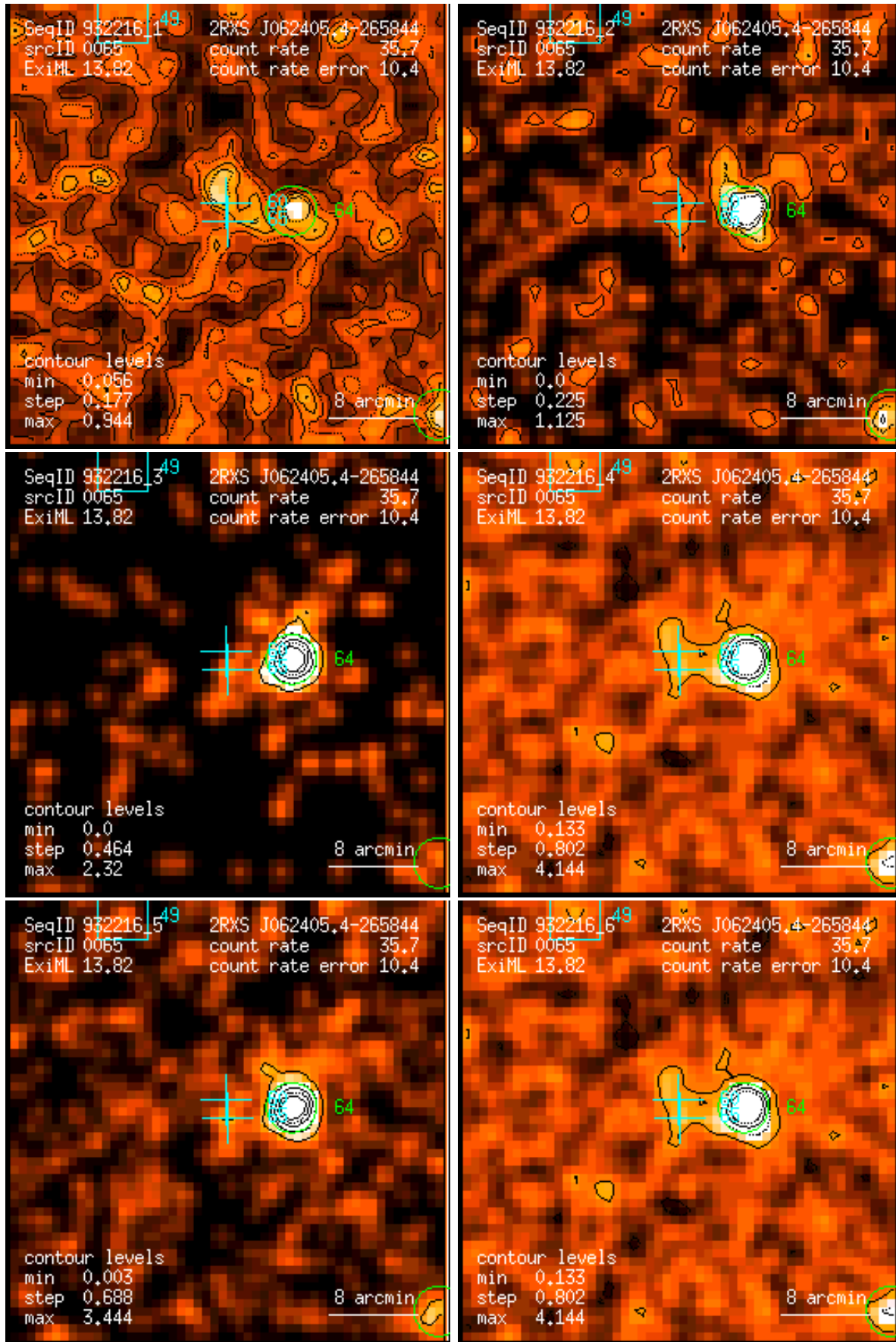
Figure 65: RASS 932216: detection 0065: band rate images, Gaussian filter: (1) PSPC channels 11 – 41, (2) 52 – 90, (3) 91 – 201, (4) 11 – 235, (5) 52 – 201, (6) 11 – 201. Broad band rates in counts/ks. Band rate contour levels in counts/ks/arcmin 2 .
