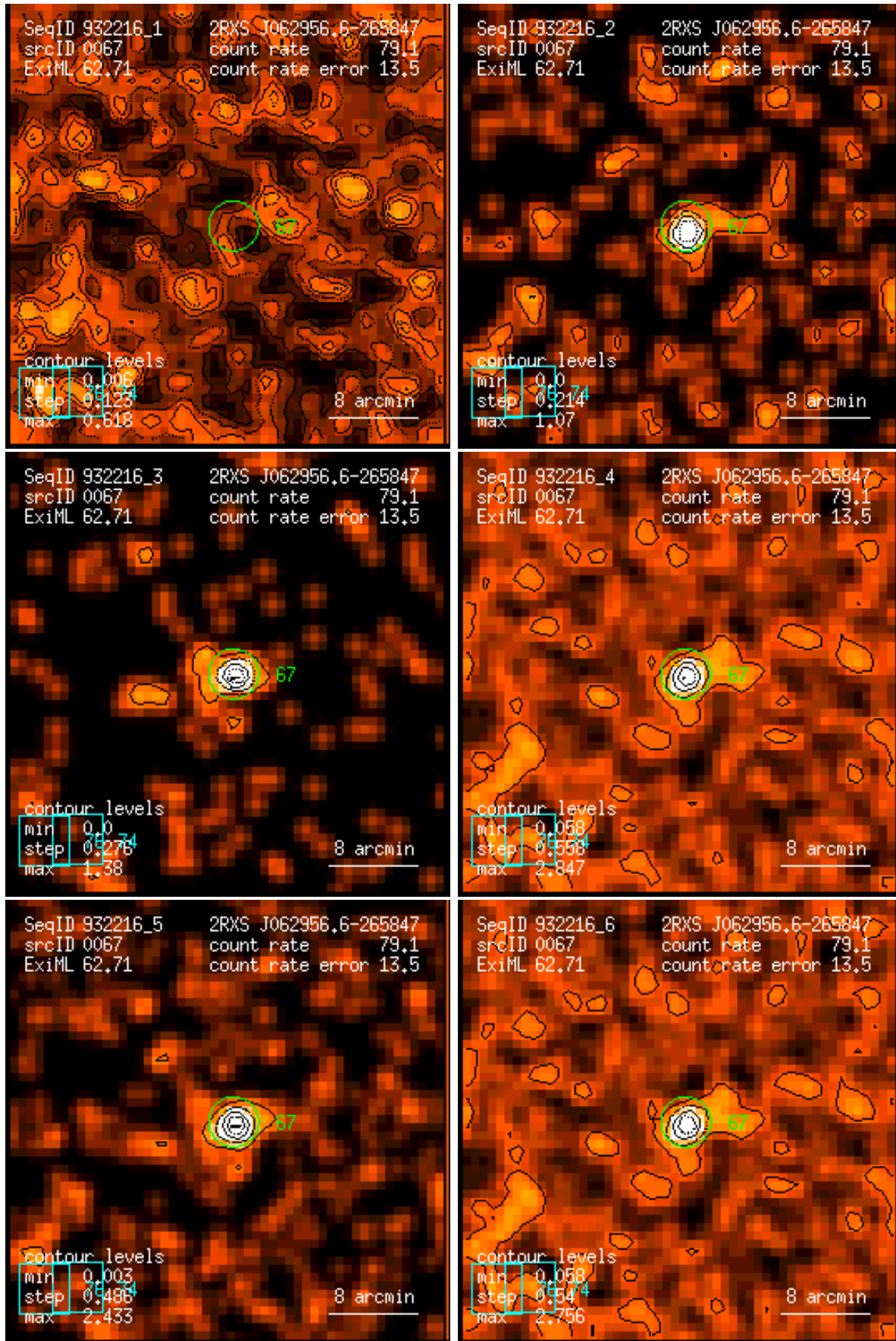
Figure 67: RASS 932216: detection 0067: band rate images, Gaussian filter: (1) PSPC channels 11 – 41, (2) 52 – 90, (3) 91 – 201, (4) 11 – 235, (5) 52 – 201, (6) 11 – 201. Broad band rates in counts/ks. Band rate contour levels in counts/ks/arcmin 2 .
