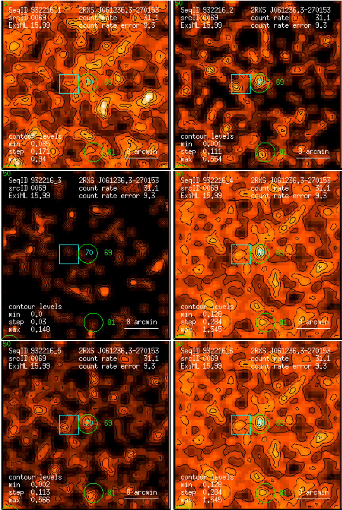
Figure 69: RASS 932216: detection 0069: band rate images, Gaussian filter: (1) PSPC channels 11 – 41, (2) 52 – 90, (3) 91 – 201, (4) 11 – 235, (5) 52 – 201, (6) 11 – 201. Broad band rates in counts/ks. Band rate contour levels in counts/ks/arcmin 2 .
