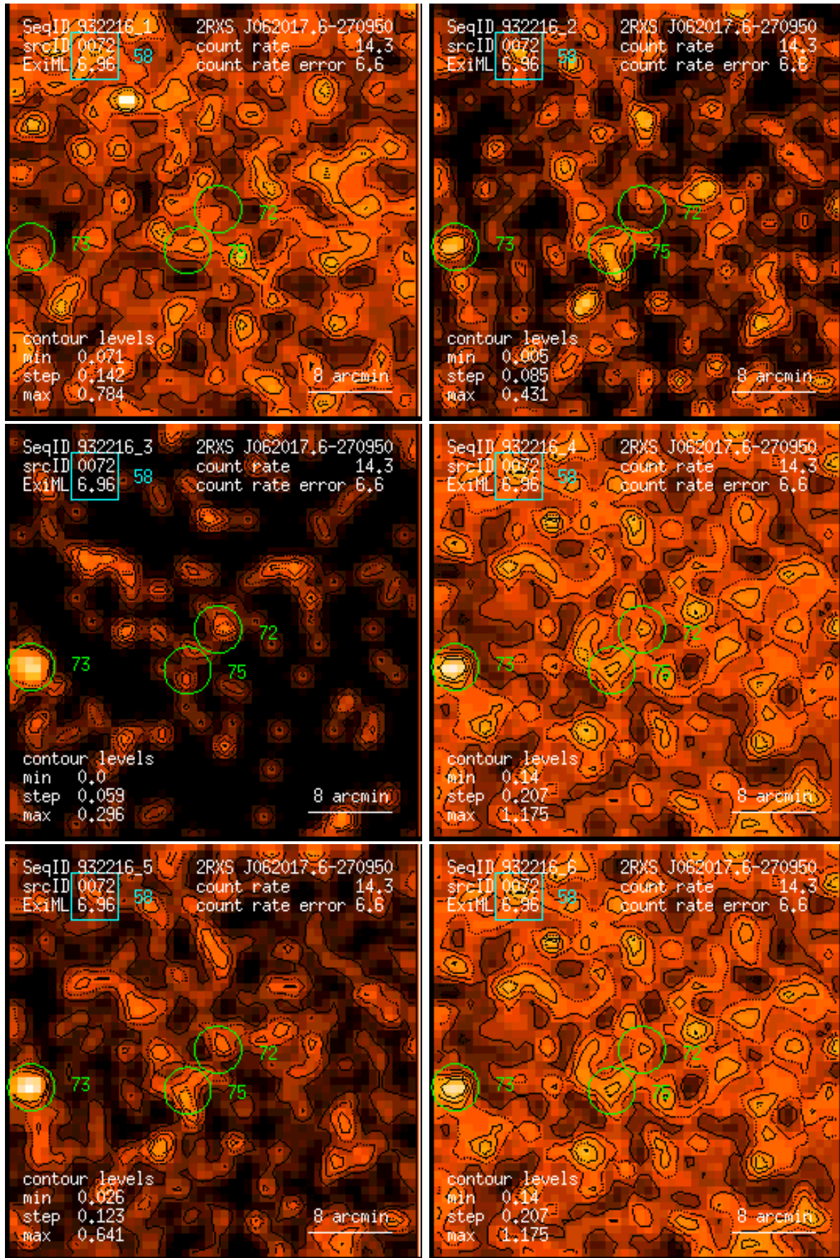
Figure 72: RASS 932216: detection 0072: band rate images, Gaussian filter: (1) PSPC channels 11 – 41, (2) 52 – 90, (3) 91 – 201, (4) 11 – 235, (5) 52 – 201, (6) 11 – 201. Broad band rates in counts/ks. Band rate contour levels in counts/ks/arcmin 2 .
