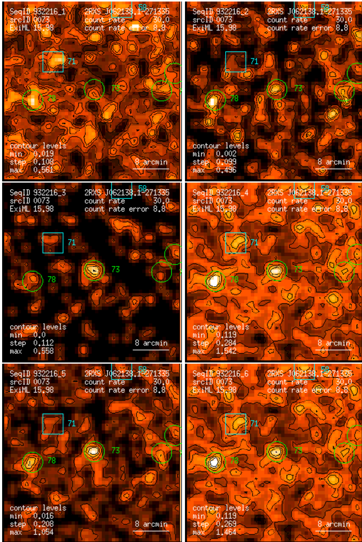
Figure 73: RASS 932216: detection 0073: band rate images, Gaussian filter: (1) PSPC channels 11 – 41, (2) 52 – 90, (3) 91 – 201, (4) 11 – 235, (5) 52 – 201, (6) 11 – 201. Broad band rates in counts/ks. Band rate contour levels in counts/ks/arcmin 2 .
