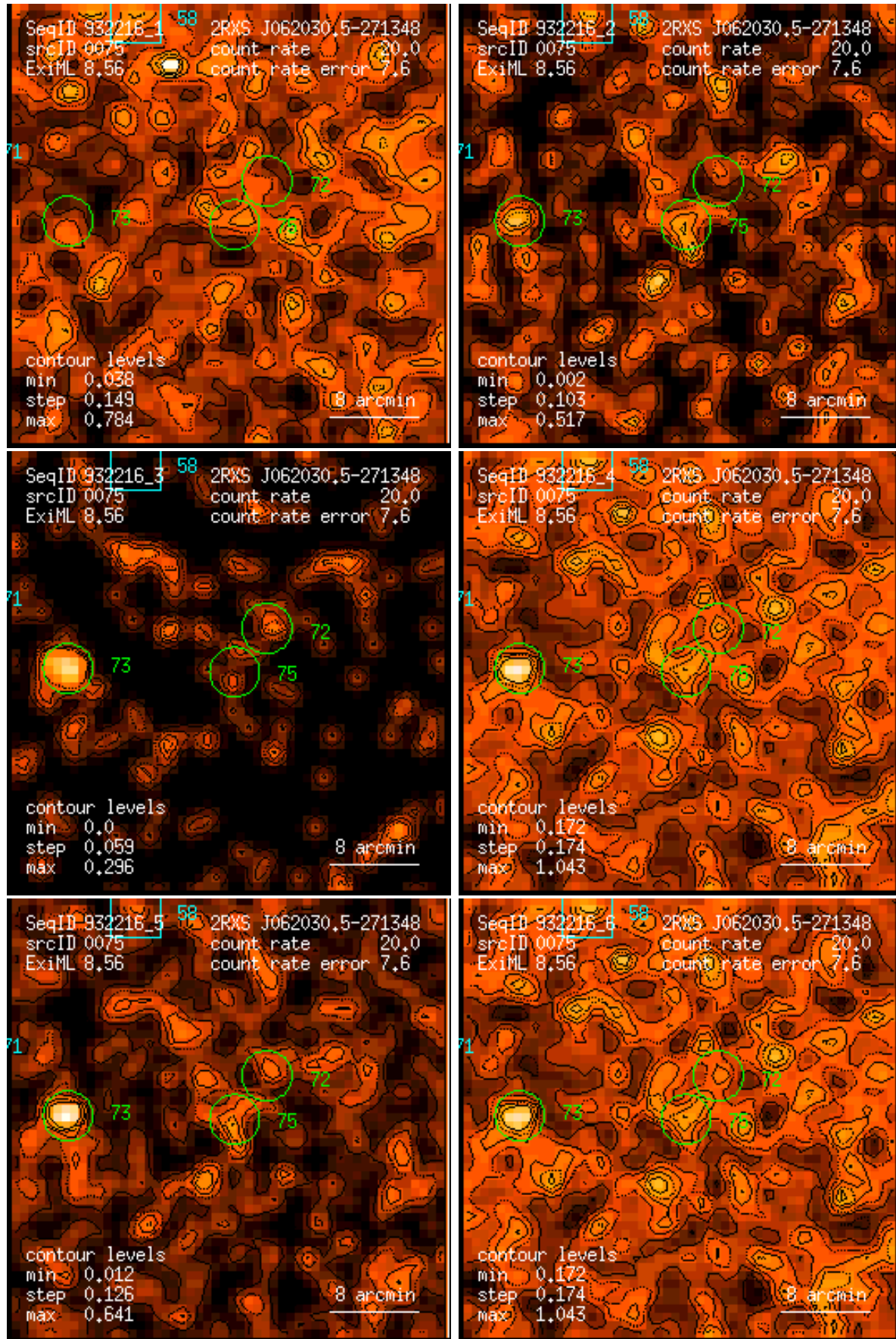
Figure 75: RASS 932216: detection 0075: band rate images, Gaussian filter: (1) PSPC channels 11 – 41, (2) 52 – 90, (3) 91 – 201, (4) 11 – 235, (5) 52 – 201, (6) 11 – 201. Broad band rates in counts/ks. Band rate contour levels in counts/ks/arcmin 2 .
