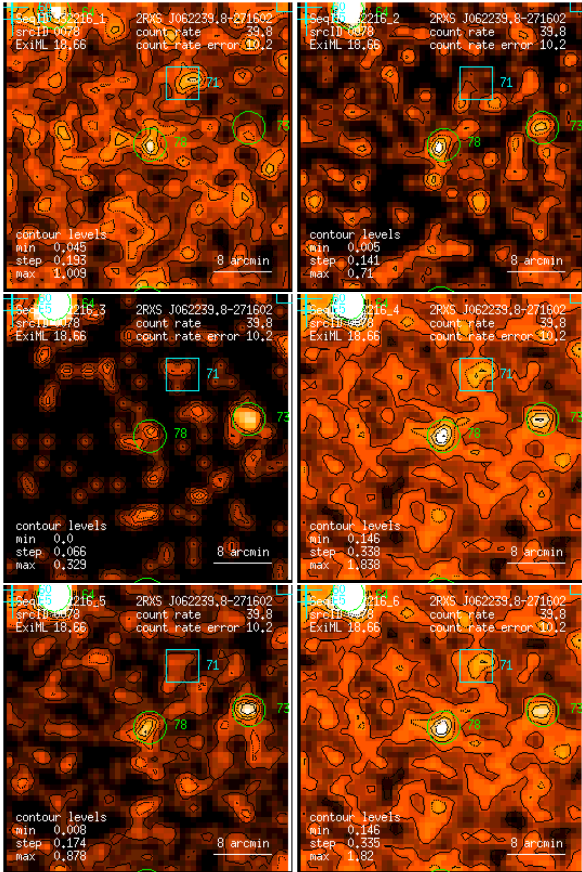
Figure 78: RASS 932216: detection 0078: band rate images, Gaussian filter: (1) PSPC channels 11 – 41, (2) 52 – 90, (3) 91 – 201, (4) 11 – 235, (5) 52 – 201, (6) 11 – 201. Broad band rates in counts/ks. Band rate contour levels in counts/ks/arcmin 2 .
