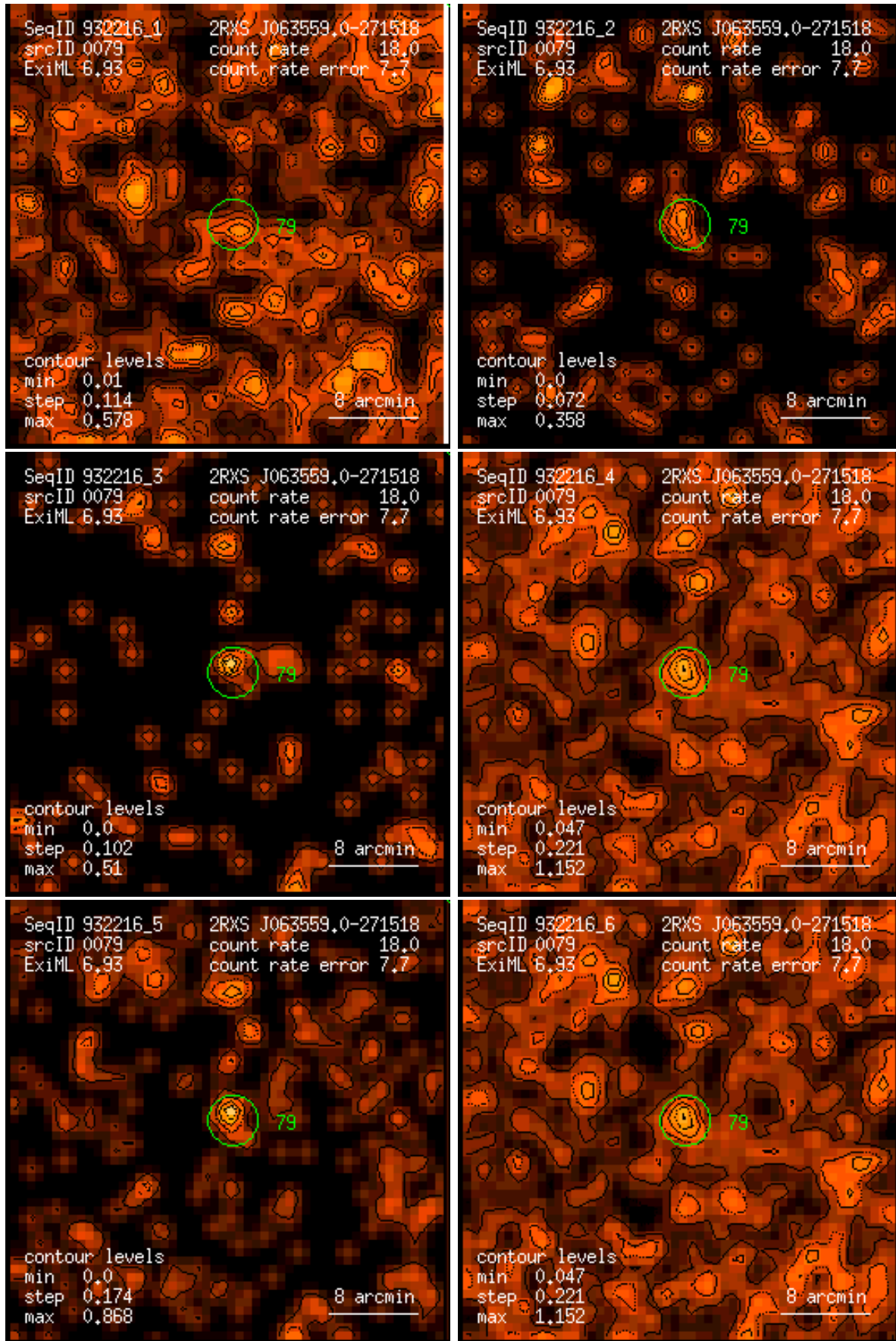
Figure 79: RASS 932216: detection 0079: band rate images, Gaussian filter: (1) PSPC channels 11 – 41, (2) 52 – 90, (3) 91 – 201, (4) 11 – 235, (5) 52 – 201, (6) 11 – 201. Broad band rates in counts/ks. Band rate contour levels in counts/ks/arcmin 2 .
