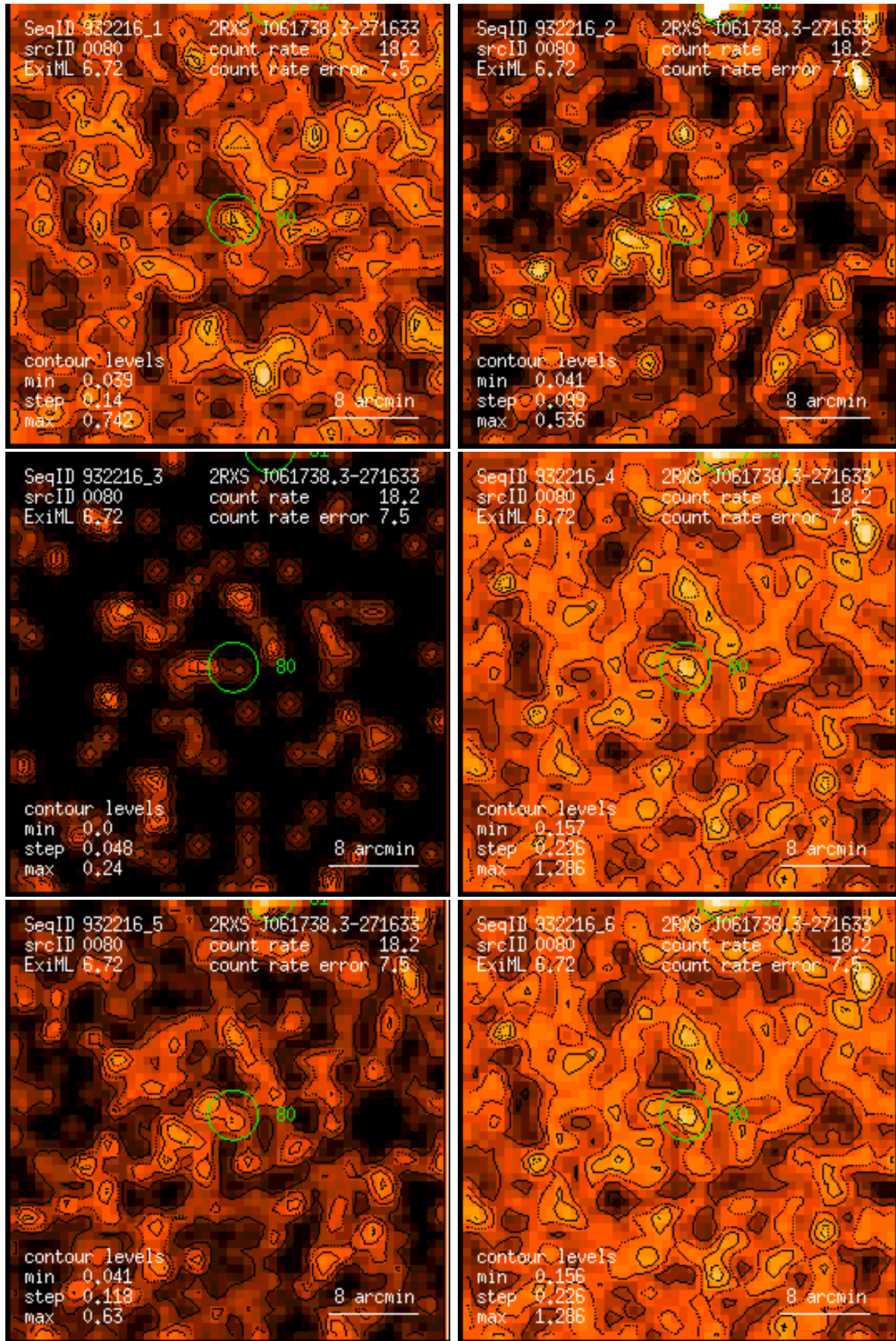
Figure 80: RASS 932216: detection 0080: band rate images, Gaussian filter: (1) PSPC channels 11 – 41, (2) 52 – 90, (3) 91 – 201, (4) 11 – 235, (5) 52 – 201, (6) 11 – 201. Broad band rates in counts/ks. Band rate contour levels in counts/ks/arcmin 2 .
