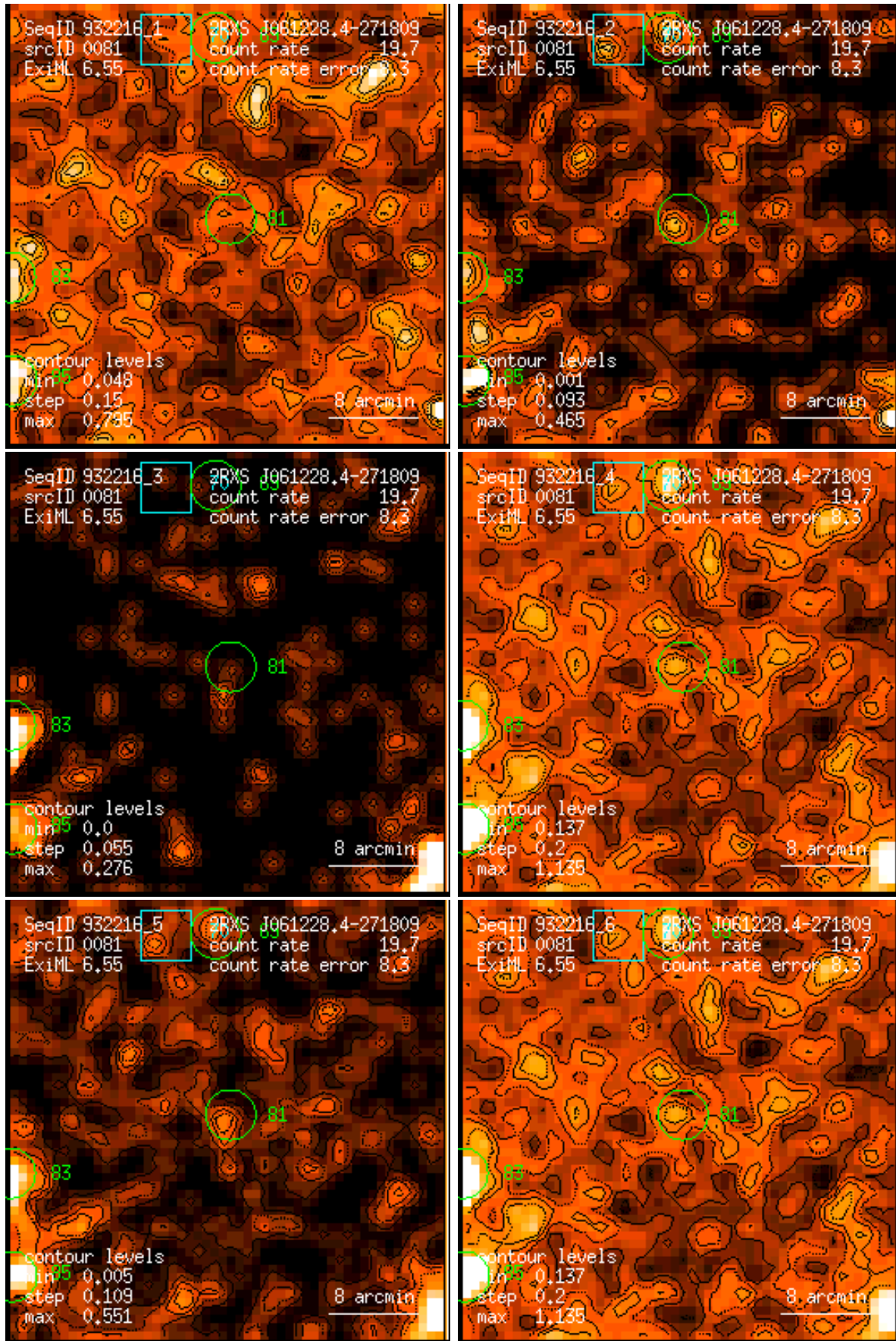
Figure 81: RASS 932216: detection 0081: band rate images, Gaussian filter: (1) PSPC channels 11 – 41, (2) 52 – 90, (3) 91 – 201, (4) 11 – 235, (5) 52 – 201, (6) 11 – 201. Broad band rates in counts/ks. Band rate contour levels in counts/ks/arcmin 2 .
