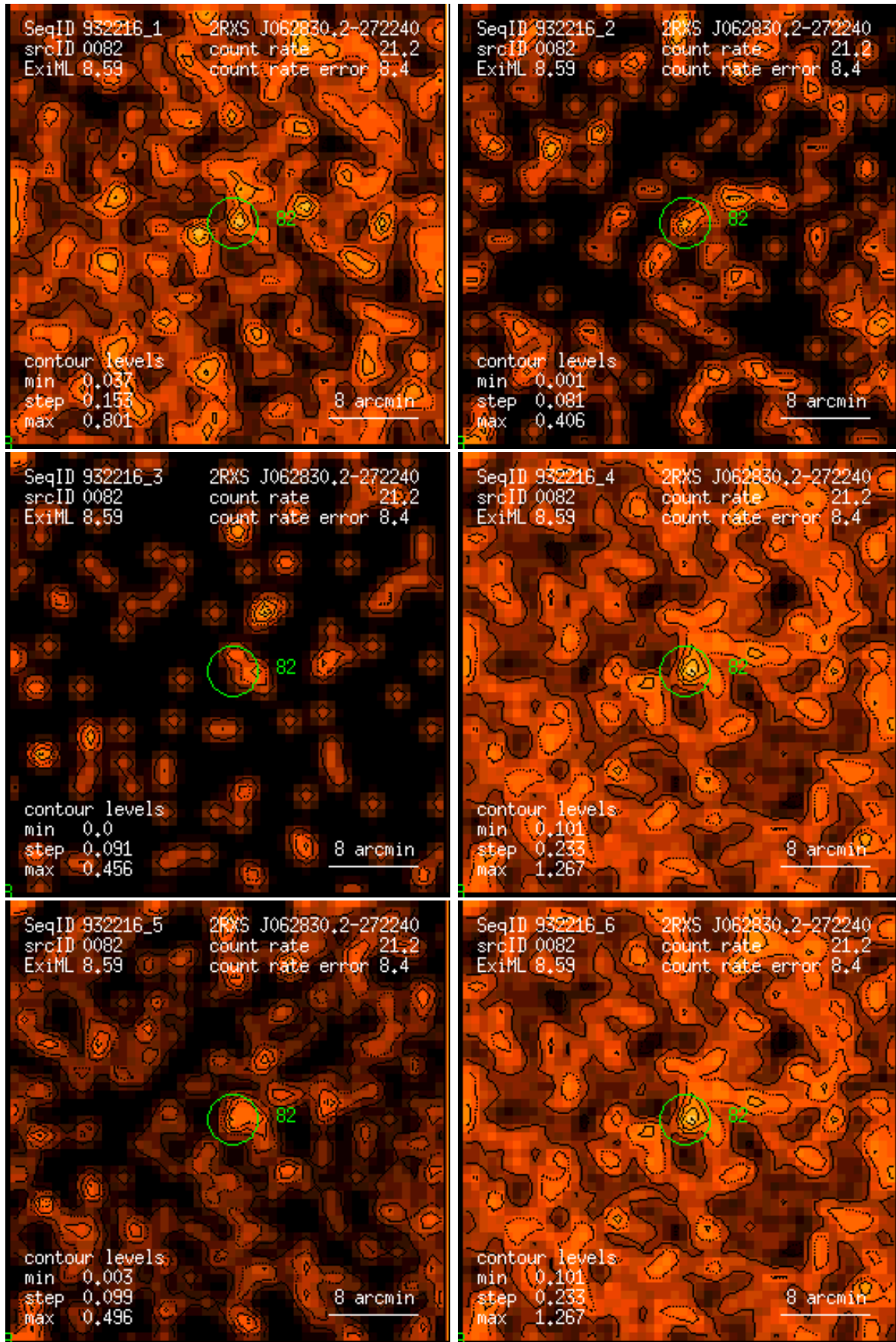
Figure 82: RASS 932216: detection 0082: band rate images, Gaussian filter: (1) PSPC channels 11 – 41, (2) 52 – 90, (3) 91 – 201, (4) 11 – 235, (5) 52 – 201, (6) 11 – 201. Broad band rates in counts/ks. Band rate contour levels in counts/ks/arcmin 2 .
