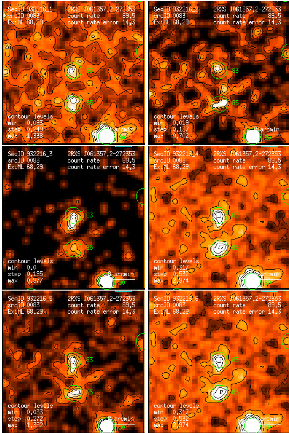
Figure 83: RASS 932216: detection 0083: band rate images, Gaussian filter: (1) PSPC channels 11 – 41, (2) 52 – 90, (3) 91 – 201, (4) 11 – 235, (5) 52 – 201, (6) 11 – 201. Broad band rates in counts/ks. Band rate contour levels in counts/ks/arcmin 2 .
