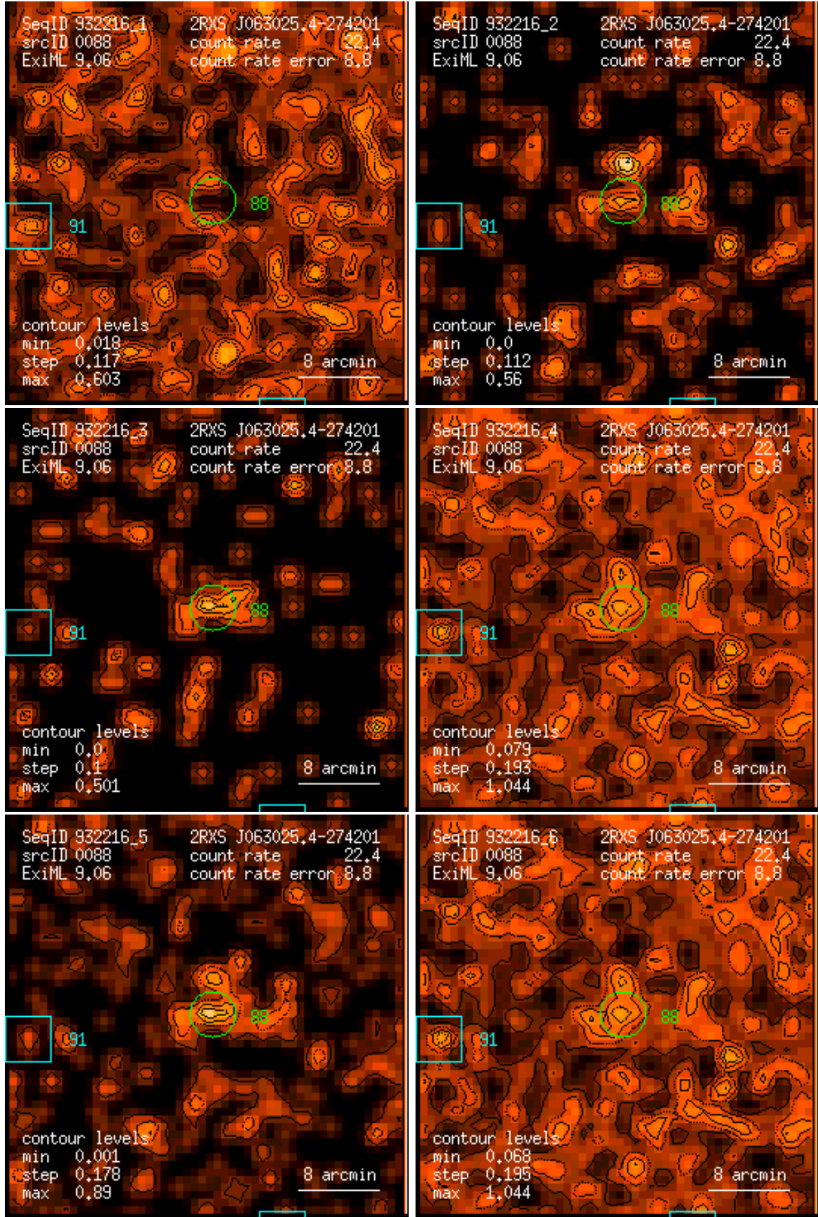
Figure 88: RASS 932216: detection 0088: band rate images, Gaussian filter: (1) PSPC channels 11 – 41, (2) 52 – 90, (3) 91 – 201, (4) 11 – 235, (5) 52 – 201, (6) 11 – 201. Broad band rates in counts/ks. Band rate contour levels in counts/ks/arcmin 2 .
