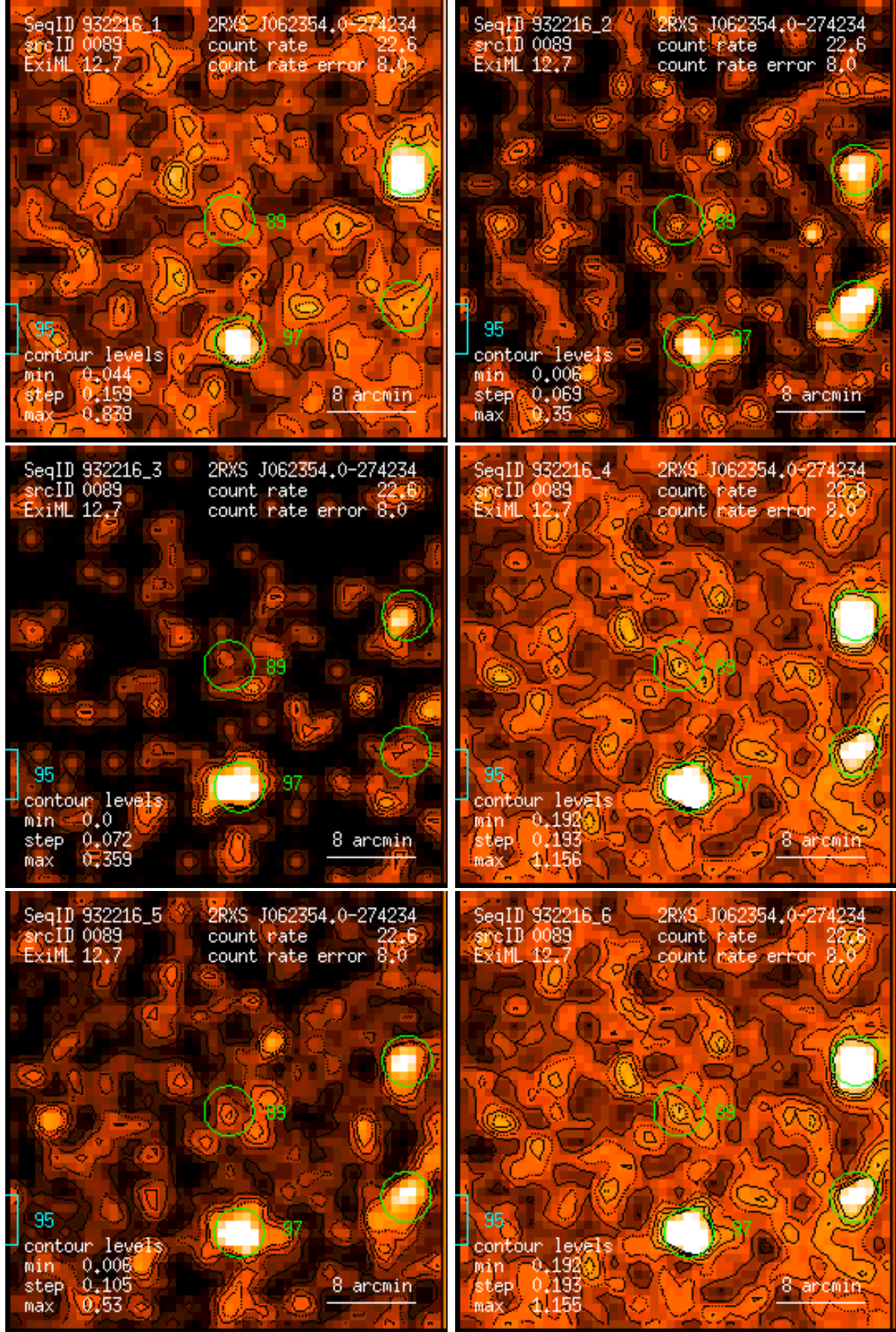
Figure 89: RASS 932216: detection 0089: band rate images, Gaussian filter: (1) PSPC channels 11 – 41, (2) 52 – 90, (3) 91 – 201, (4) 11 – 235, (5) 52 – 201, (6) 11 – 201. Broad band rates in counts/ks. Band rate contour levels in counts/ks/arcmin 2 .
