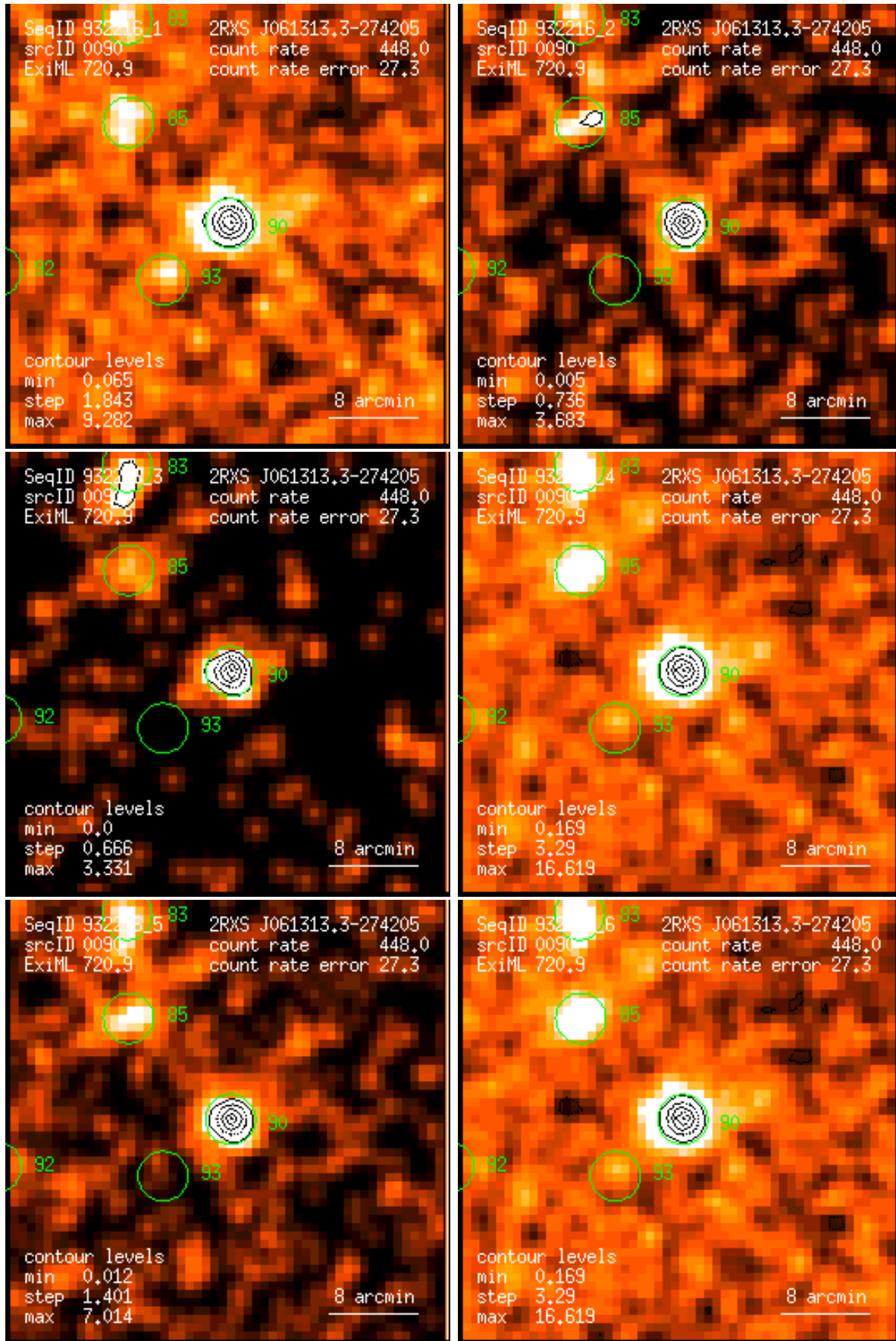
Figure 90: RASS 932216: detection 0090: band rate images, Gaussian filter: (1) PSPC channels 11 – 41, (2) 52 – 90, (3) 91 – 201, (4) 11 – 235, (5) 52 – 201, (6) 11 – 201. Broad band rates in counts/ks. Band rate contour levels in counts/ks/arcmin 2 .
