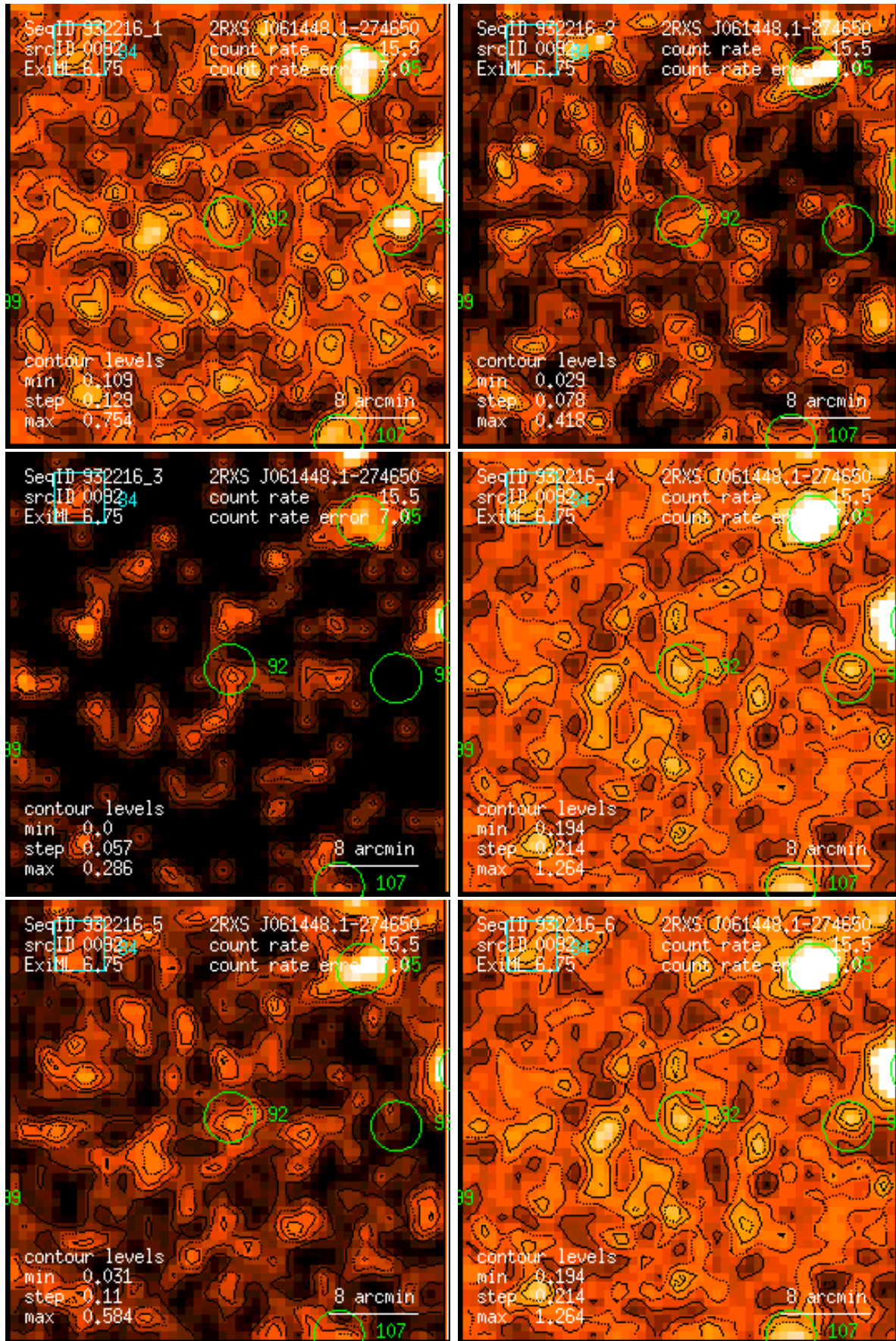
Figure 92: RASS 932216: detection 0092: band rate images, Gaussian filter: (1) PSPC channels 11 – 41, (2) 52 – 90, (3) 91 – 201, (4) 11 – 235, (5) 52 – 201, (6) 11 – 201. Broad band rates in counts/ks. Band rate contour levels in counts/ks/arcmin 2 .
