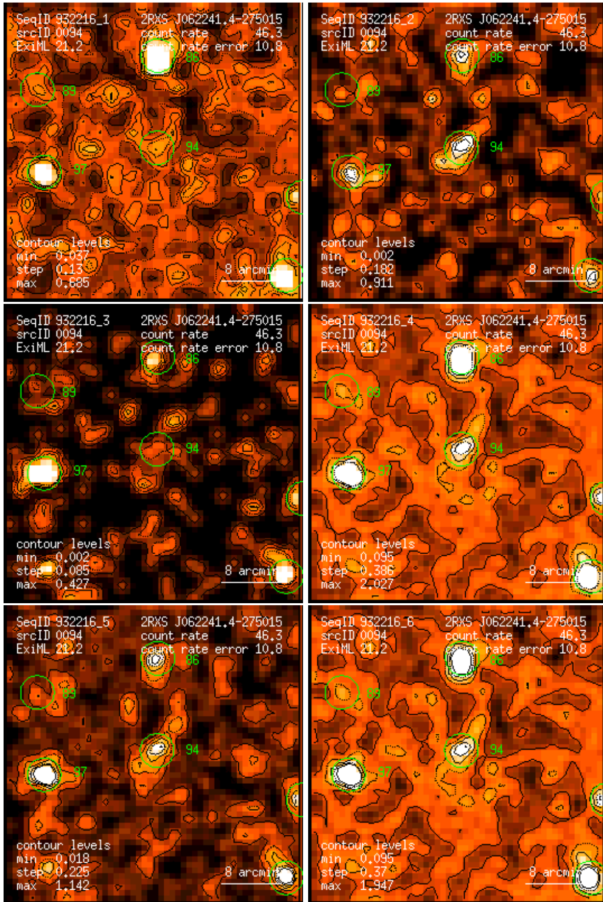
Figure 94: RASS 932216: detection 0094: band rate images, Gaussian filter: (1) PSPC channels 11 – 41, (2) 52 – 90, (3) 91 – 201, (4) 11 – 235, (5) 52 – 201, (6) 11 – 201. Broad band rates in counts/ks. Band rate contour levels in counts/ks/arcmin 2 .
