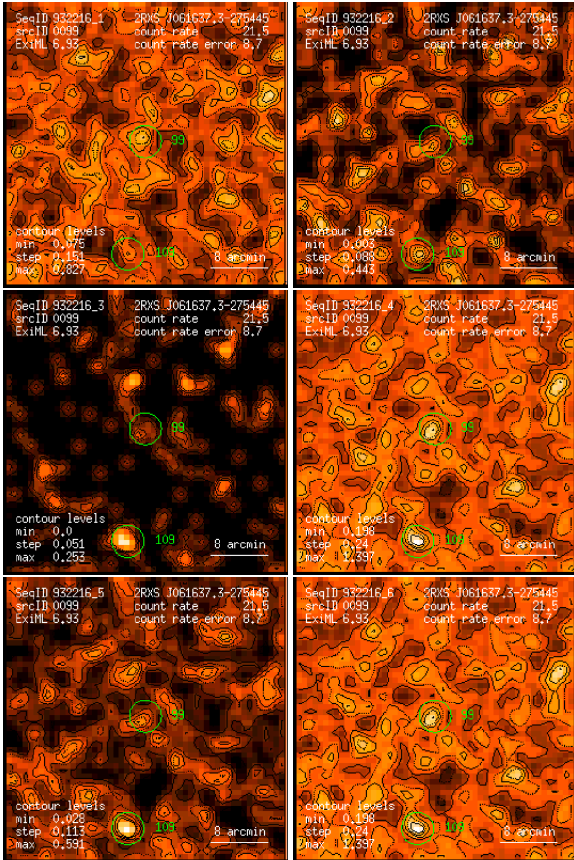
Figure 99: RASS 932216: detection 0099: band rate images, Gaussian filter: (1) PSPC channels 11 – 41, (2) 52 – 90, (3) 91 – 201, (4) 11 – 235, (5) 52 – 201, (6) 11 – 201. Broad band rates in counts/ks. Band rate contour levels in counts/ks/arcmin 2 .
