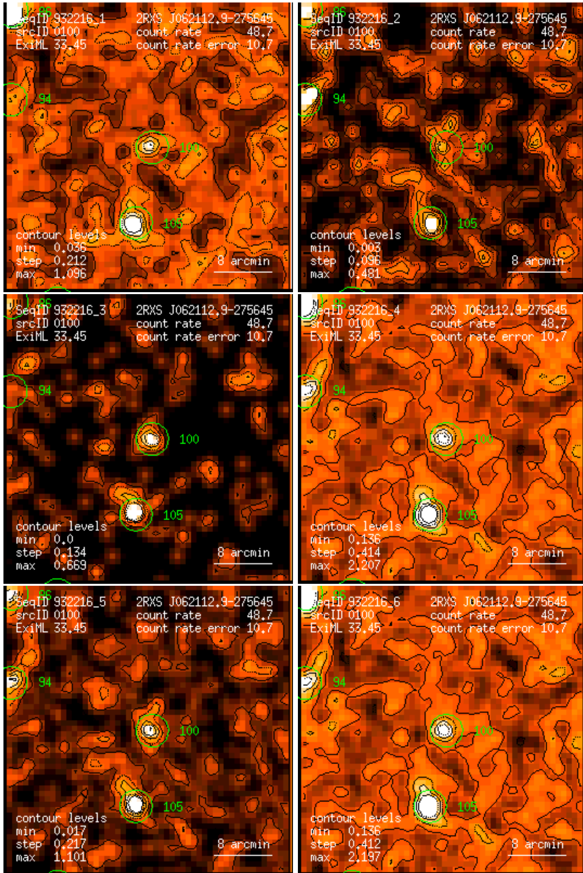
Figure 100: RASS 932216: detection 0100: band rate images, Gaussian filter: (1) PSPC channels 11 – 41, (2) 52 – 90, (3) 91 – 201, (4) 11 – 235, (5) 52 – 201, (6) 11 – 201. Broad band rates in counts/ks. Band rate contour levels in counts/ks/arcmin 2 .
