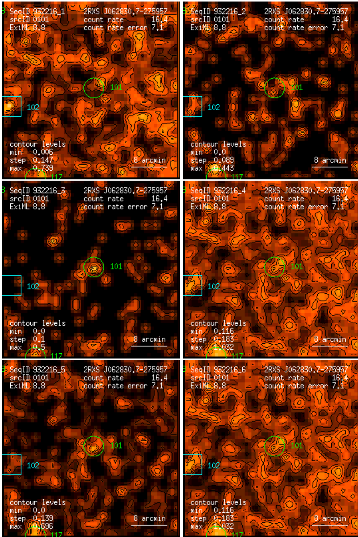
Figure 101: RASS 932216: detection 0101: band rate images, Gaussian filter: (1) PSPC channels 11 – 41, (2) 52 – 90, (3) 91 – 201, (4) 11 – 235, (5) 52 – 201, (6) 11 – 201. Broad band rates in counts/ks. Band rate contour levels in counts/ks/arcmin 2 .
