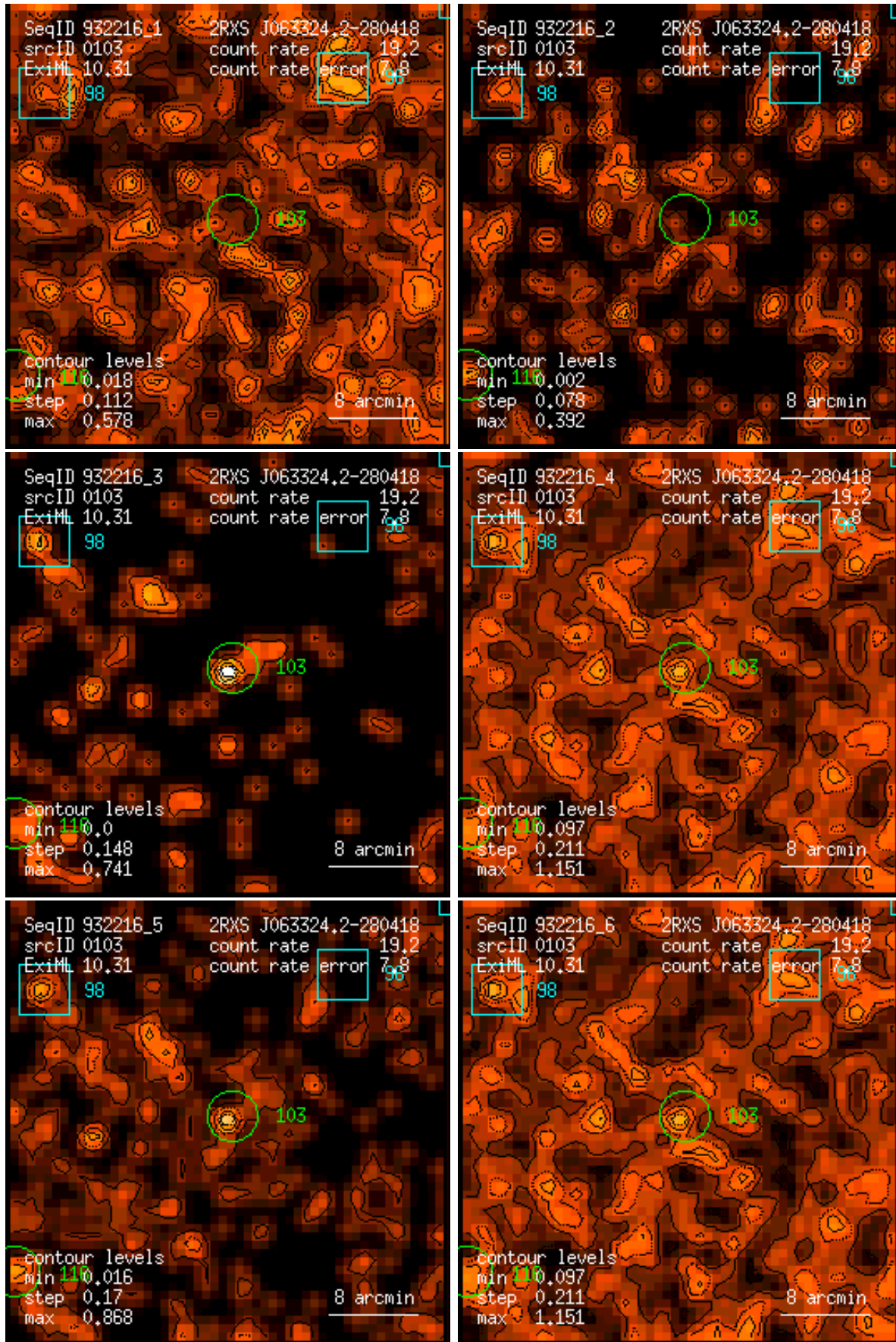
Figure 103: RASS 932216: detection 0103: band rate images, Gaussian filter: (1) PSPC channels 11 – 41, (2) 52 – 90, (3) 91 – 201, (4) 11 – 235, (5) 52 – 201, (6) 11 – 201. Broad band rates in counts/ks. Band rate contour levels in counts/ks/arcmin 2 .
