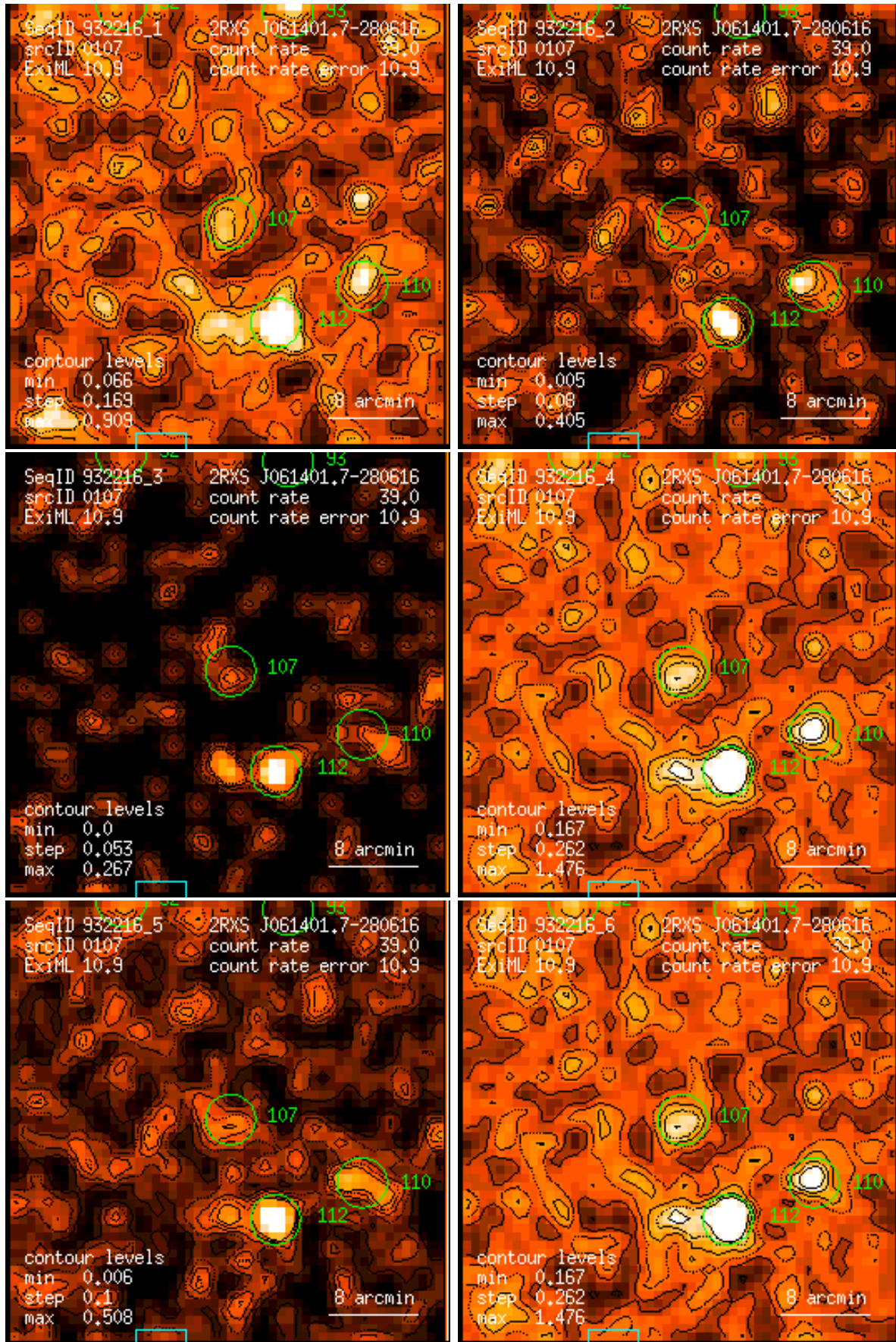
Figure 107: RASS 932216: detection 0107: band rate images, Gaussian filter: (1) PSPC channels 11 – 41, (2) 52 – 90, (3) 91 – 201, (4) 11 – 235, (5) 52 – 201, (6) 11 – 201. Broad band rates in counts/ks. Band rate contour levels in counts/ks/arcmin 2 .
