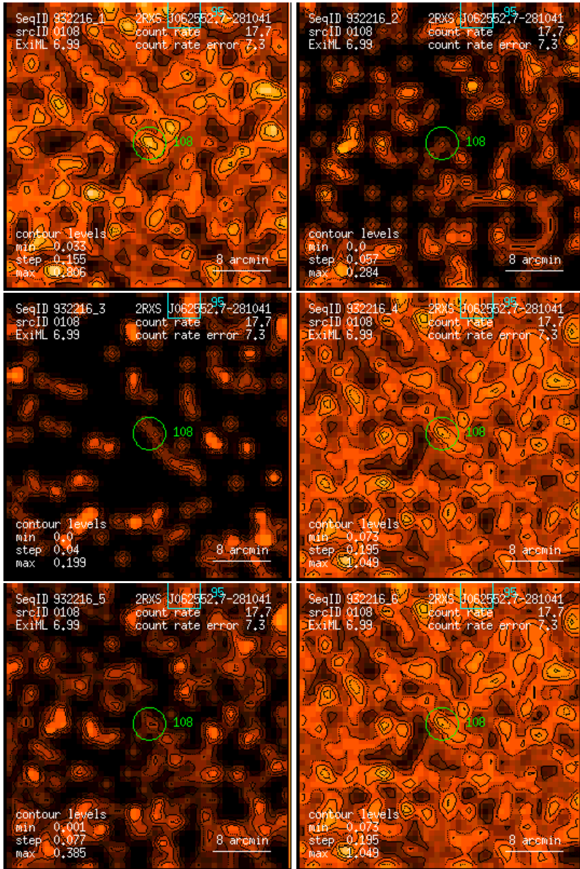
Figure 108: RASS 932216: detection 0108: band rate images, Gaussian filter: (1) PSPC channels 11 – 41, (2) 52 – 90, (3) 91 – 201, (4) 11 – 235, (5) 52 – 201, (6) 11 – 201. Broad band rates in counts/ks. Band rate contour levels in counts/ks/arcmin 2 .
