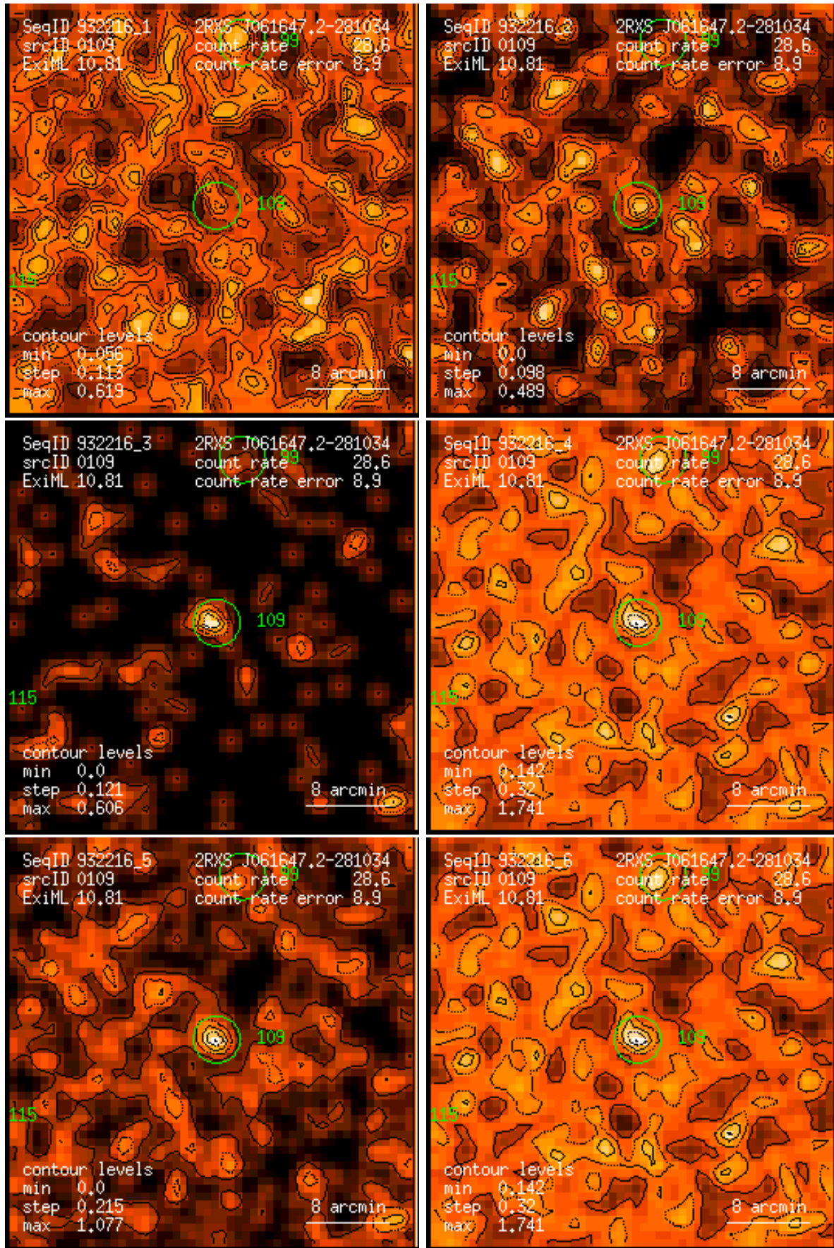
Figure 109: RASS 932216: detection 0109: band rate images, Gaussian filter: (1) PSPC channels 11 – 41, (2) 52 – 90, (3) 91 – 201, (4) 11 – 235, (5) 52 – 201, (6) 11 – 201. Broad band rates in counts/ks. Band rate contour levels in counts/ks/arcmin 2 .
