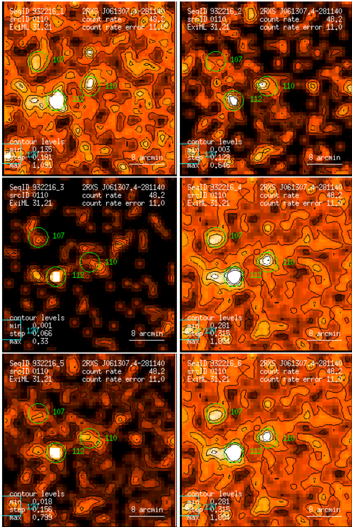
Figure 110: RASS 932216: detection 0110: band rate images, Gaussian filter: (1) PSPC channels 11 – 41, (2) 52 – 90, (3) 91 – 201, (4) 11 – 235, (5) 52 – 201, (6) 11 – 201. Broad band rates in counts/ks. Band rate contour levels in counts/ks/arcmin 2 .
