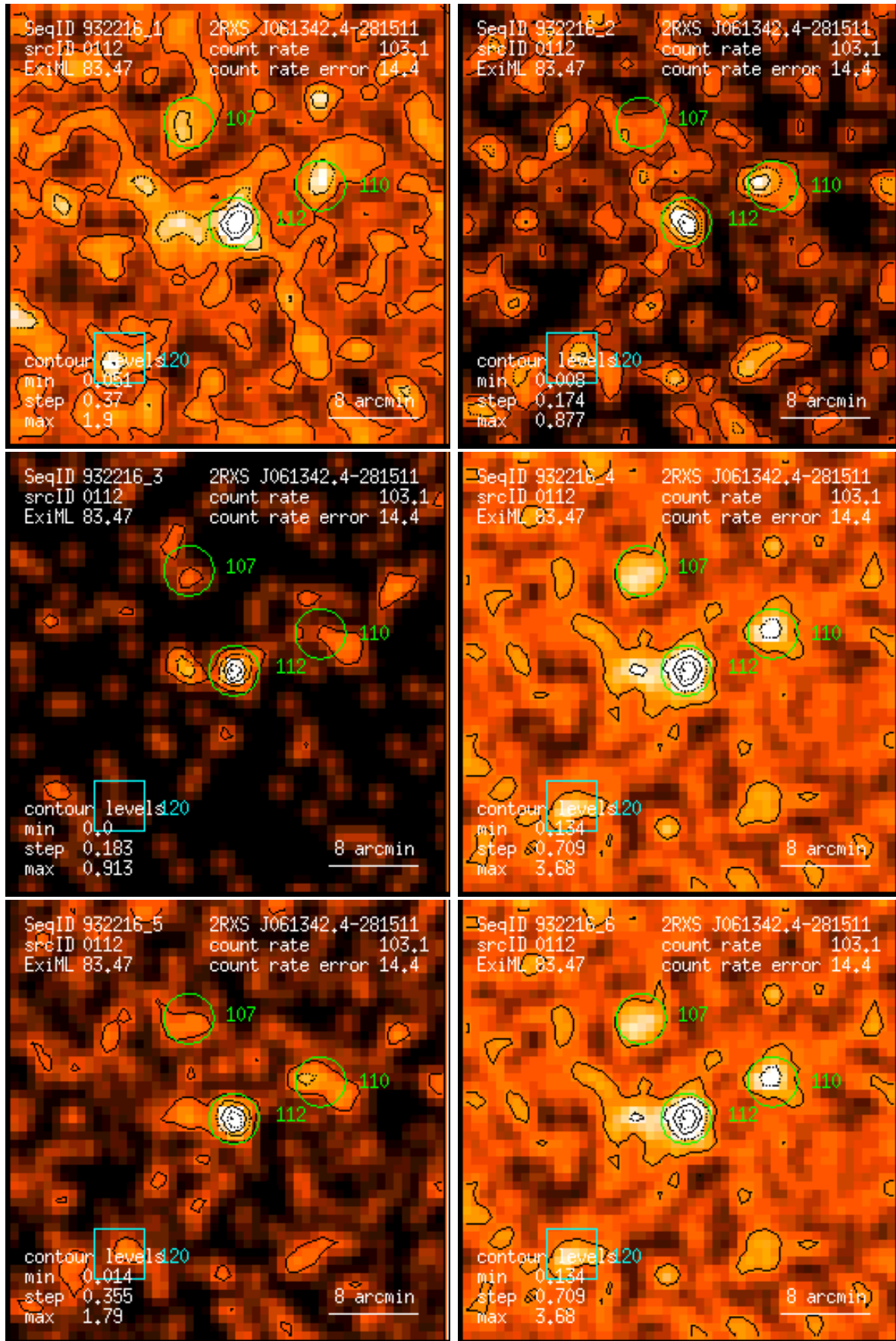
Figure 112: RASS 932216: detection 0112: band rate images, Gaussian filter: (1) PSPC channels 11 – 41, (2) 52 – 90, (3) 91 – 201, (4) 11 – 235, (5) 52 – 201, (6) 11 – 201. Broad band rates in counts/ks. Band rate contour levels in counts/ks/arcmin 2 .
