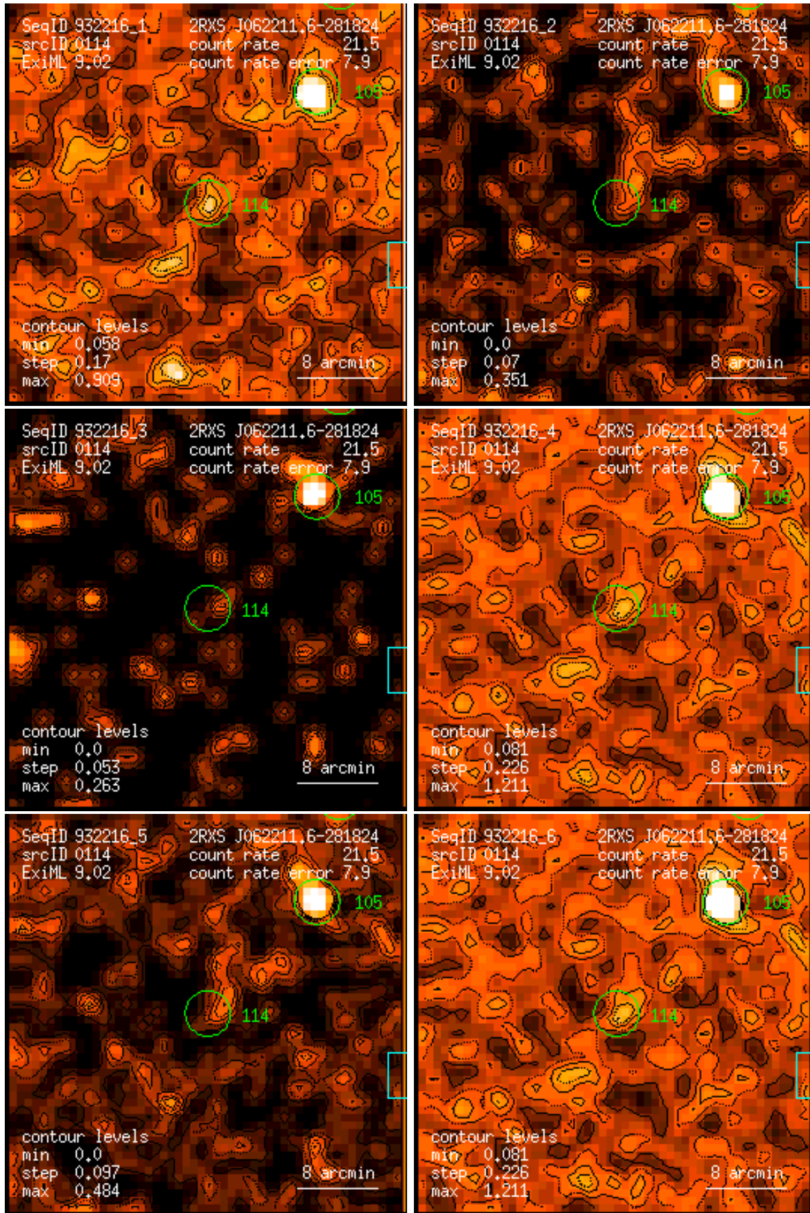
Figure 114: RASS 932216: detection 0114: band rate images, Gaussian filter: (1) PSPC channels 11 – 41, (2) 52 – 90, (3) 91 – 201, (4) 11 – 235, (5) 52 – 201, (6) 11 – 201. Broad band rates in counts/ks. Band rate contour levels in counts/ks/arcmin 2 .
