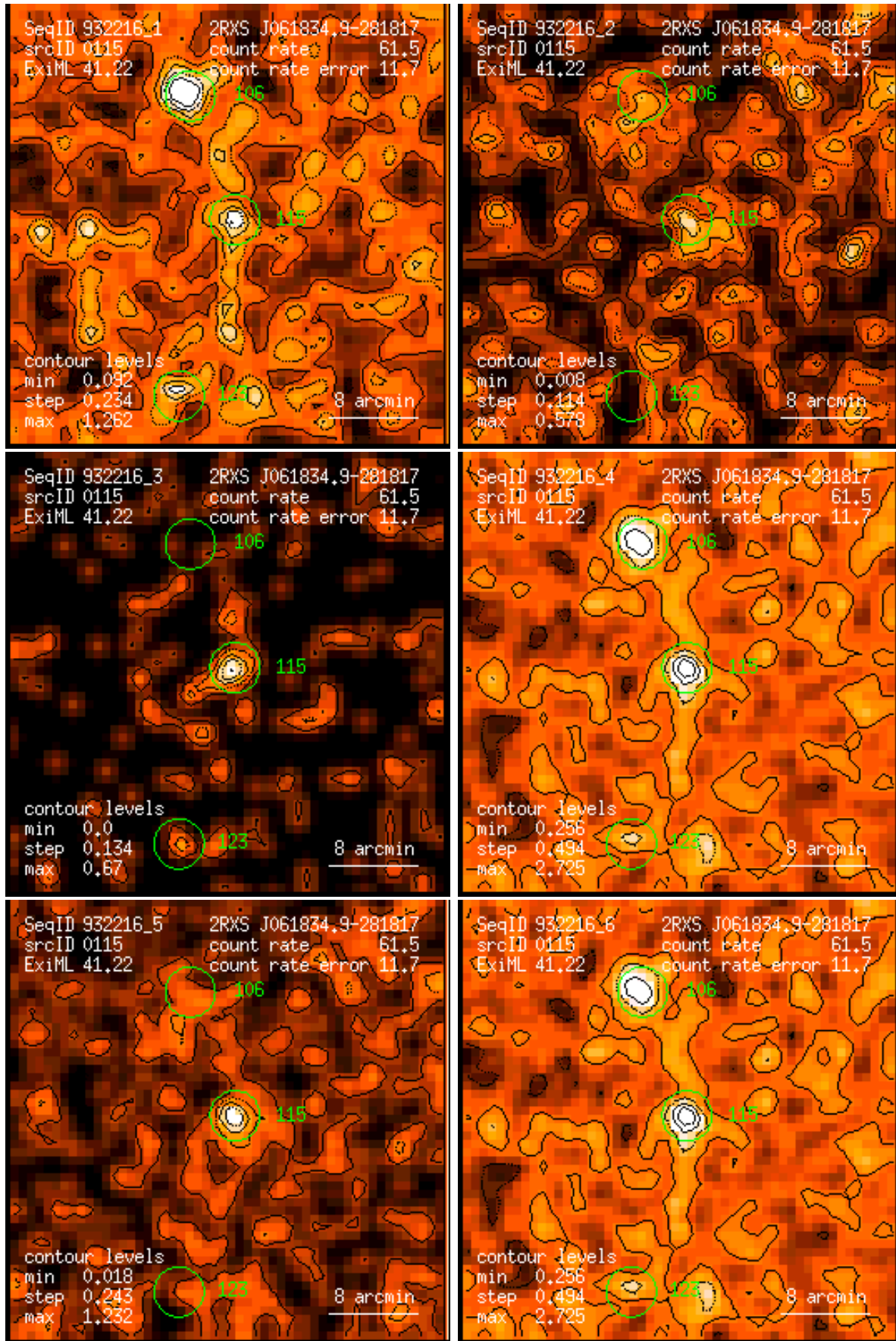
Figure 115: RASS 932216: detection 0115: band rate images, Gaussian filter: (1) PSPC channels 11 – 41, (2) 52 – 90, (3) 91 – 201, (4) 11 – 235, (5) 52 – 201, (6) 11 – 201. Broad band rates in counts/ks. Band rate contour levels in counts/ks/arcmin 2 .
