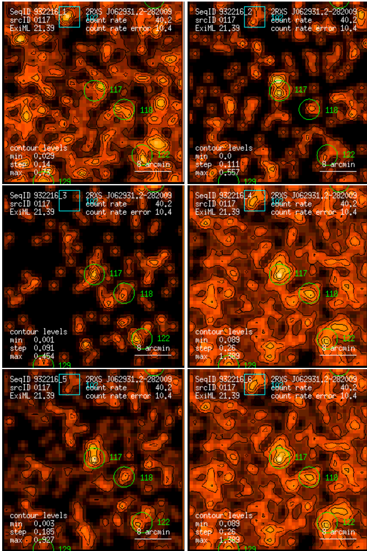
Figure 117: RASS 932216: detection 0117: band rate images, Gaussian filter: (1) PSPC channels 11 – 41, (2) 52 – 90, (3) 91 – 201, (4) 11 – 235, (5) 52 – 201, (6) 11 – 201. Broad band rates in counts/ks. Band rate contour levels in counts/ks/arcmin 2 .
