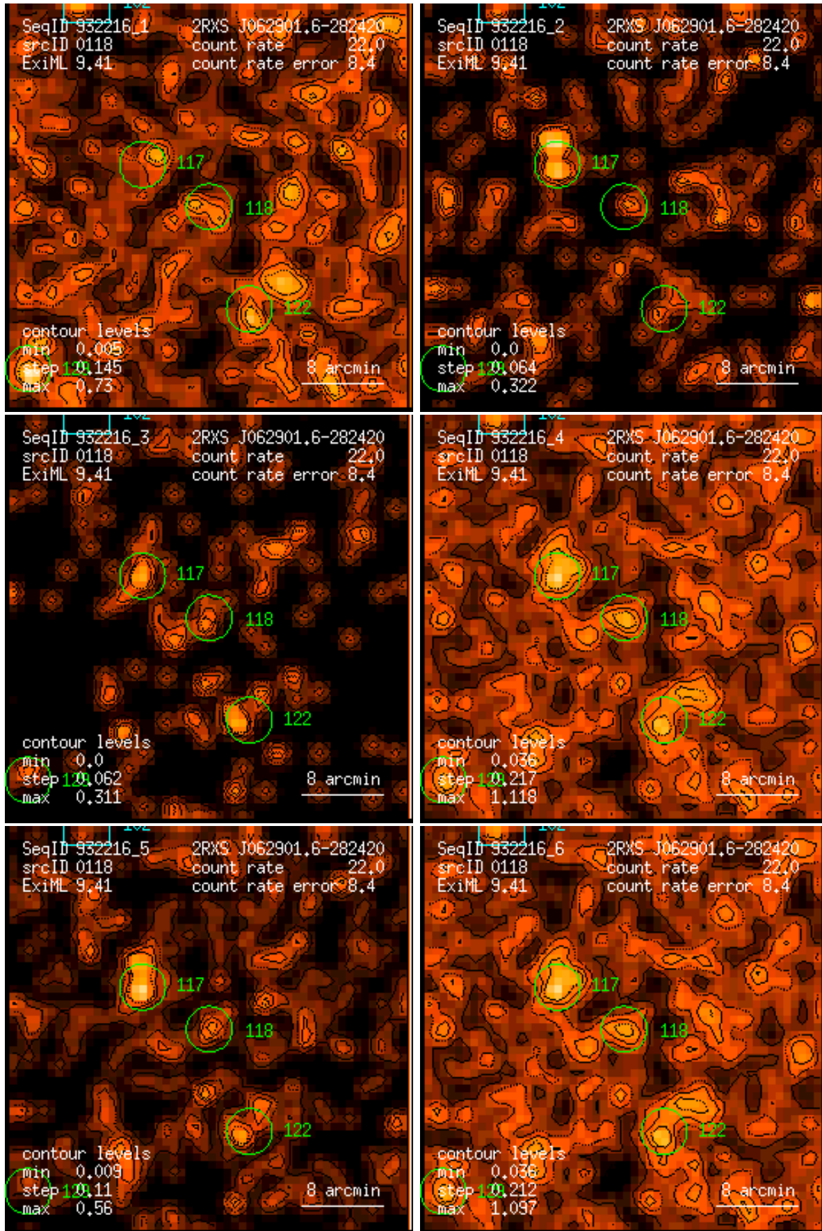
Figure 118: RASS 932216: detection 0118: band rate images, Gaussian filter: (1) PSPC channels 11 – 41, (2) 52 – 90, (3) 91 – 201, (4) 11 – 235, (5) 52 – 201, (6) 11 – 201. Broad band rates in counts/ks. Band rate contour levels in counts/ks/arcmin 2 .
